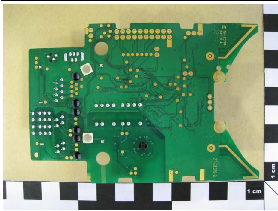
PCB Back
