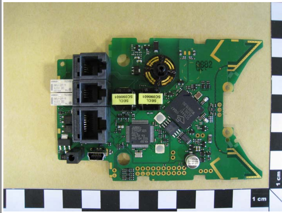
PCB Front
