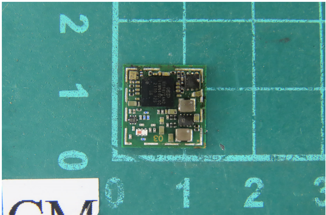
(26) EUT Photo
