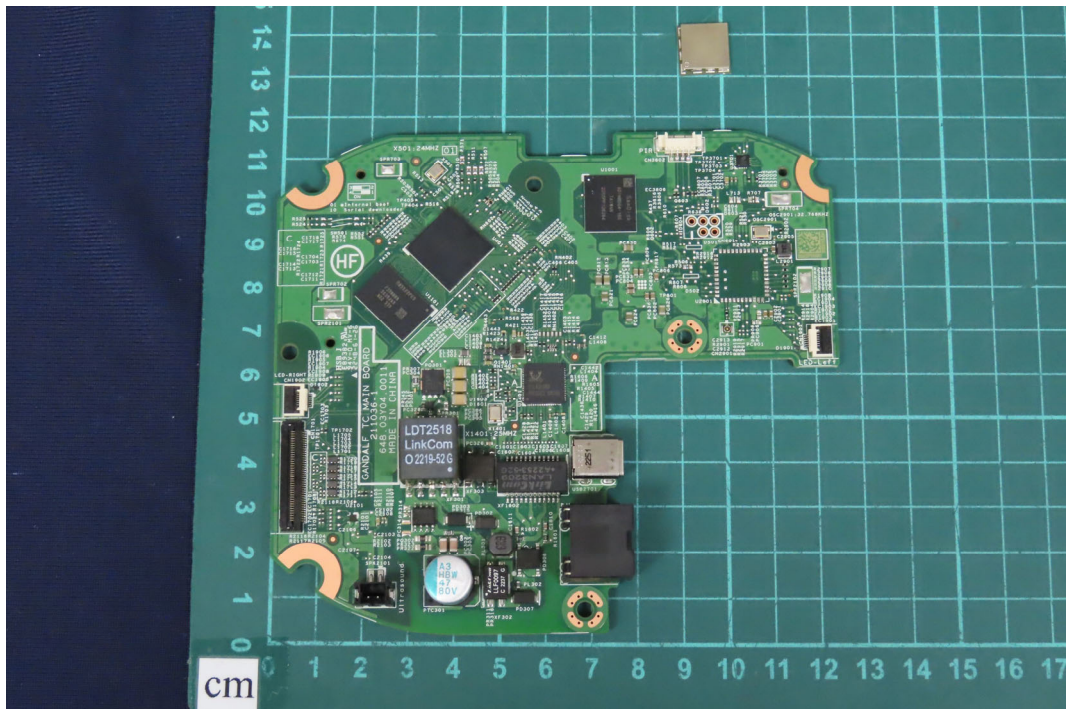
(23) EUT Photo
