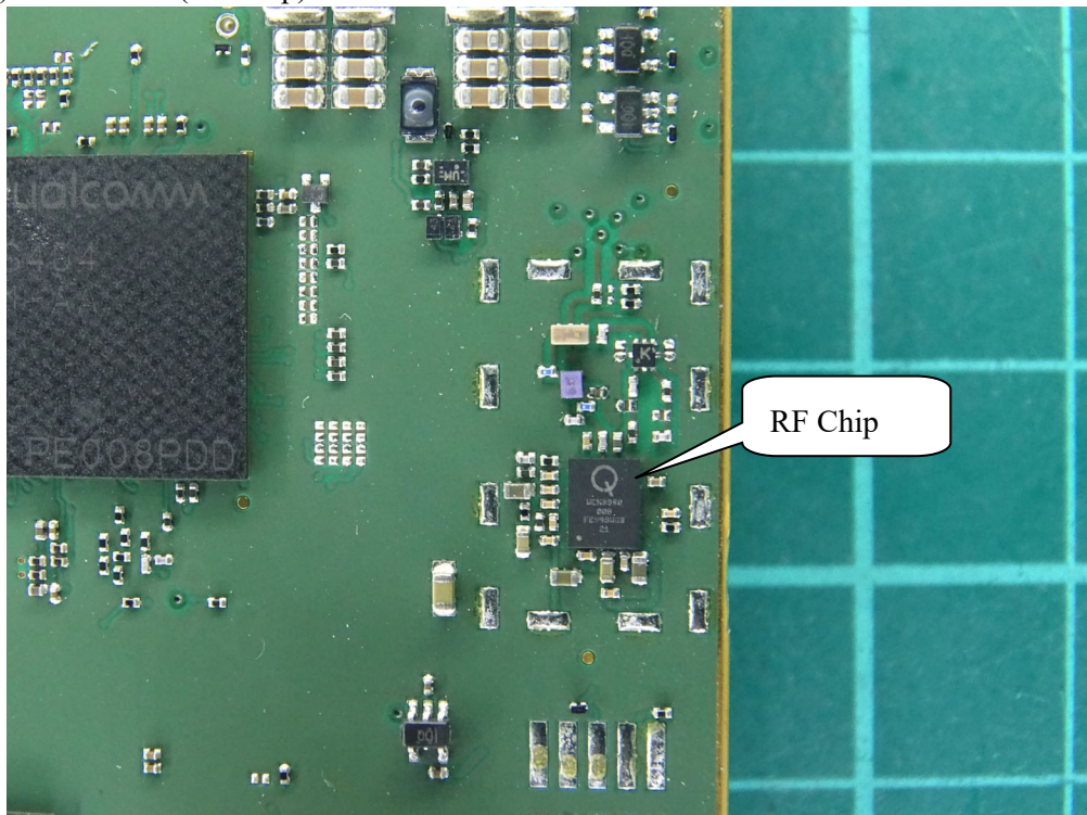
(28) EUT Photo (RF Chip)
