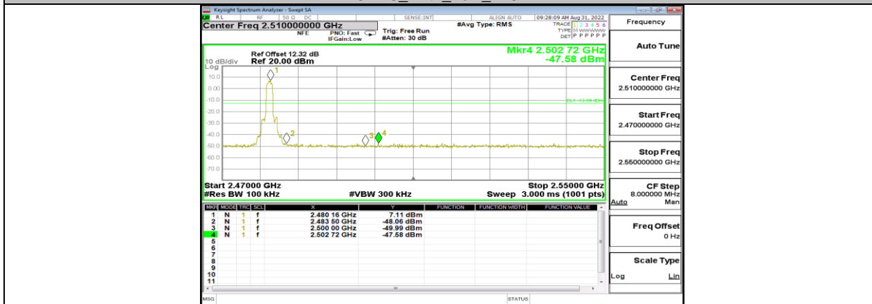
3DH5_Ant1_High_2480
