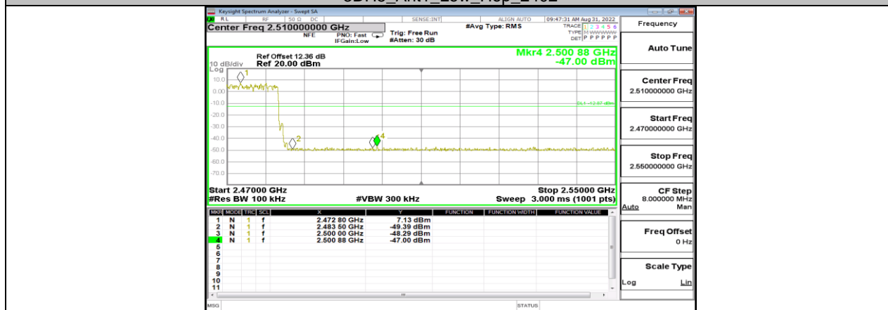
3DH5_Ant1_High_Hop_2480
