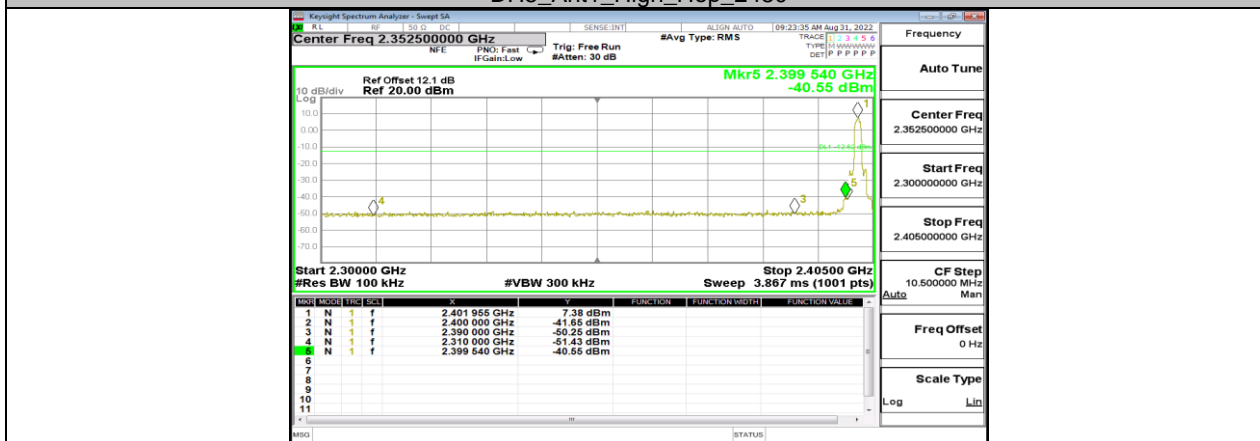
3DH5_Ant1_Low_2402
