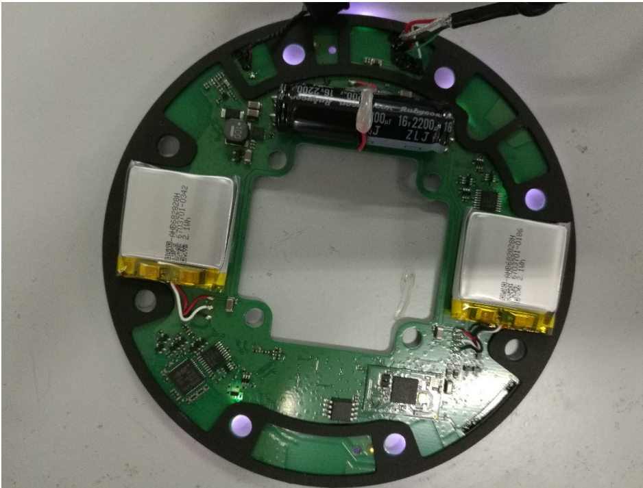
PHS040W Internal Photos (2/3)
