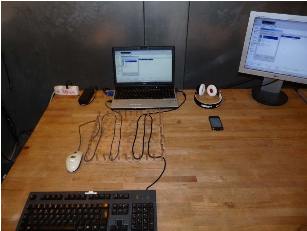
Photo 1: Test setup for conducted measurements (AC Port (power line), computer peripheral setup, EUT supplied by USB-cable from computer, intentional / unintentional radiator §15) Computer supplied by 110v 60Hz AC.
