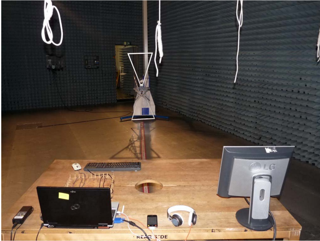
Photo 2: Test setup for radiated measurements (computer peripheral setup, EUT supplied by USB-cable from computer, unintentional radiator S15)
