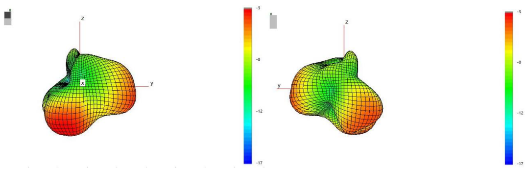
Left- Antenna
