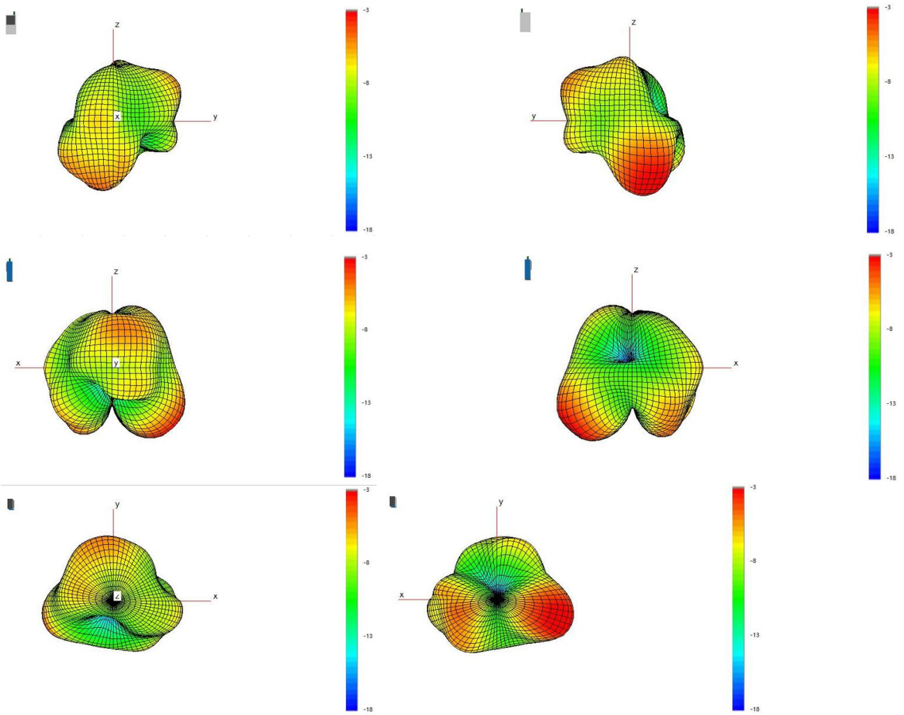
Right- Antenna
