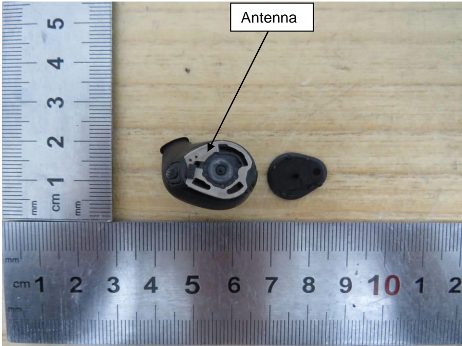
Internal View of EUT-1-L
