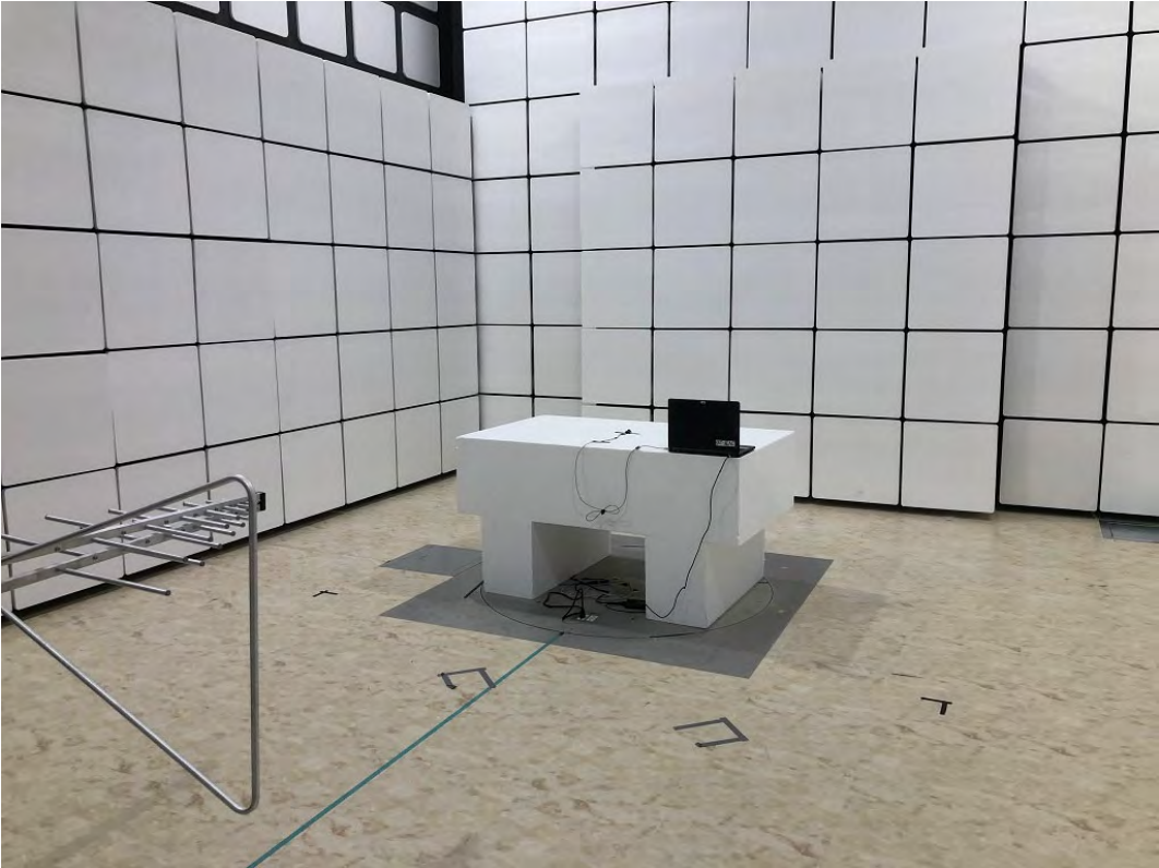
Radiated Test - OTE140R
