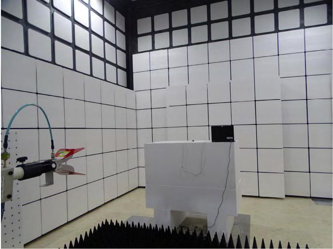
Radiated Test (Horn) -OTE140L
