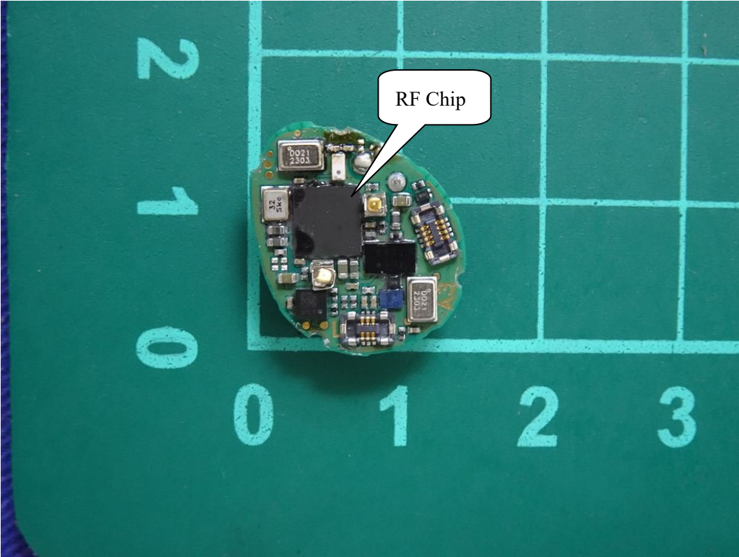
(68) EUT Photo
