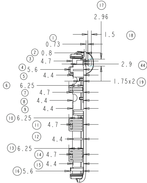
SECTION Y-Y
