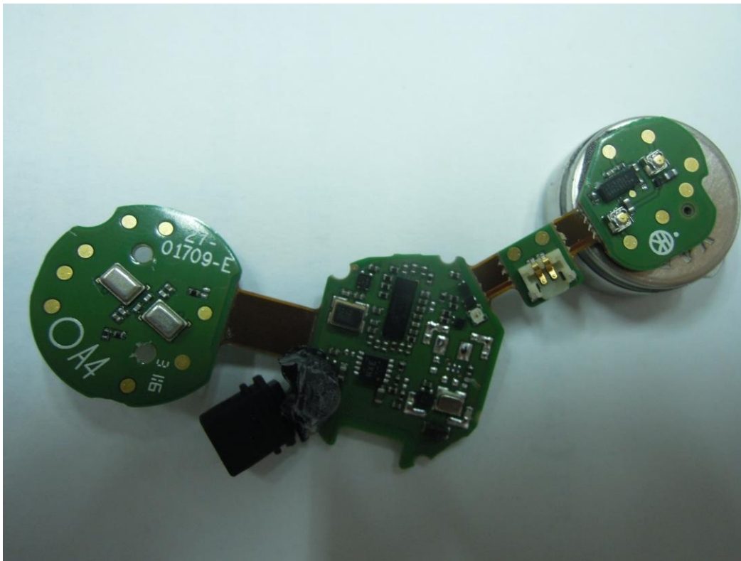
Jabra Elite Left earbud – Internal photos- Model: OTE051
