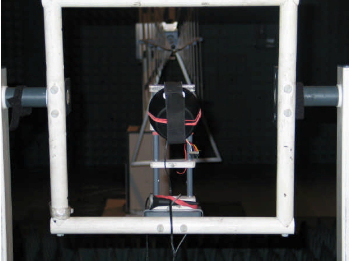
Photo 1: Test setup for radiated measurements (above 1 GHz)
