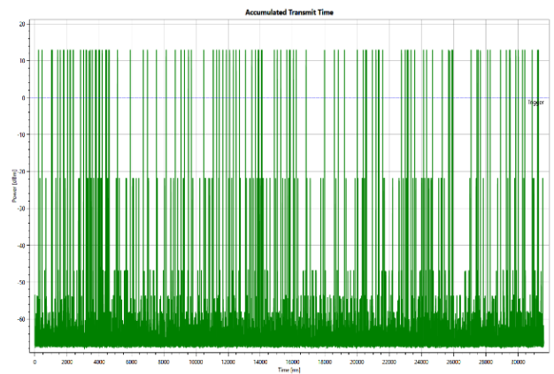
Hopping of Number
