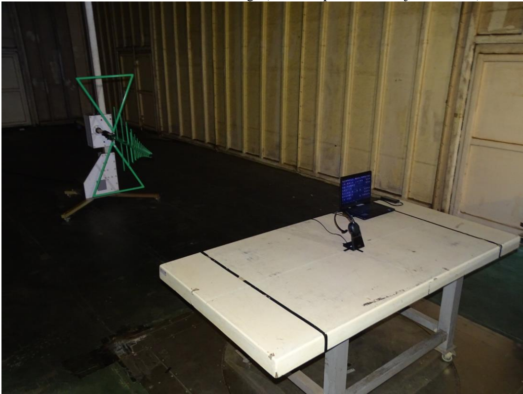
Back View of Radiated Test _Charge (mono earphone with adjustable arm)
