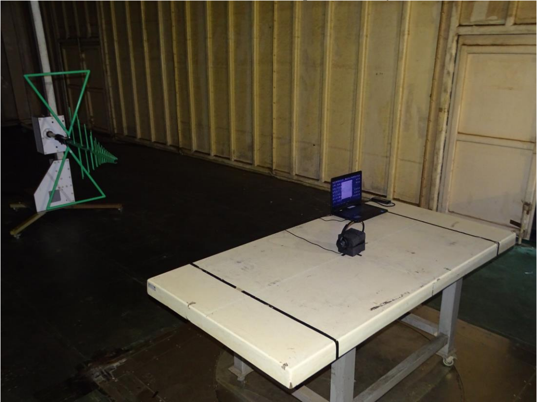
Front View of Radiated Test (mono earphone with adjustable arm)
