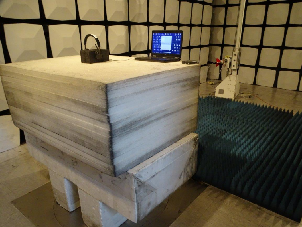
Front View of Radiated Test (Horn) (stereo headset with adjustable arm)
