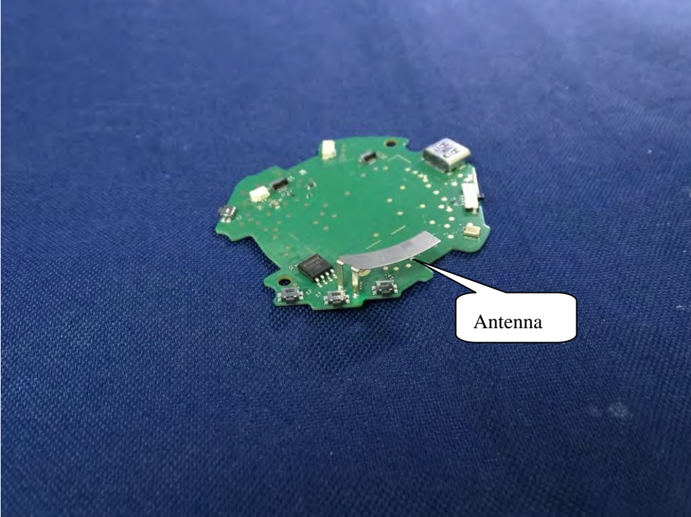
(28) EUT Photo _ANT (stereo headset with adjustable arm)
