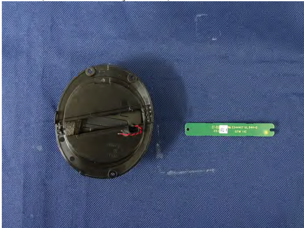
(17) EUT Photo (stereo headset with adjustable arm)
