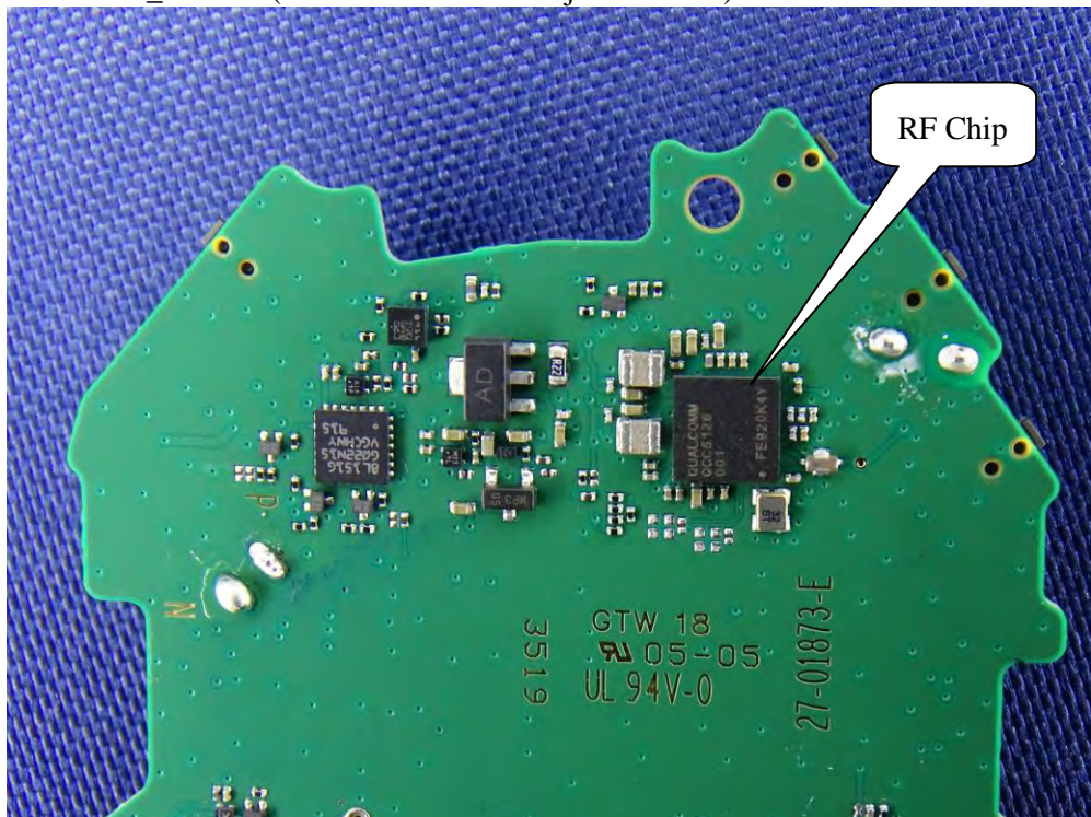
(30) EUT Photo _Module (stereo headset with adjustable arm)
