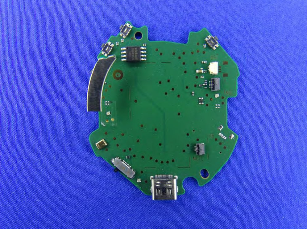
(50) EUT Photo (mono earphone with adjustable arm)
