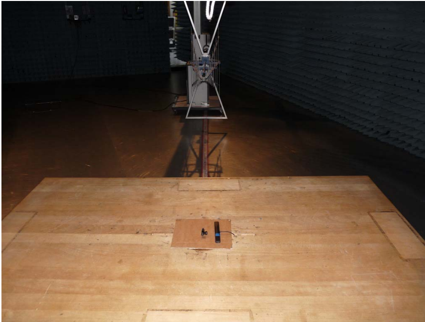
Photo 10: FCC 15c Radiated 30-1000MHz
