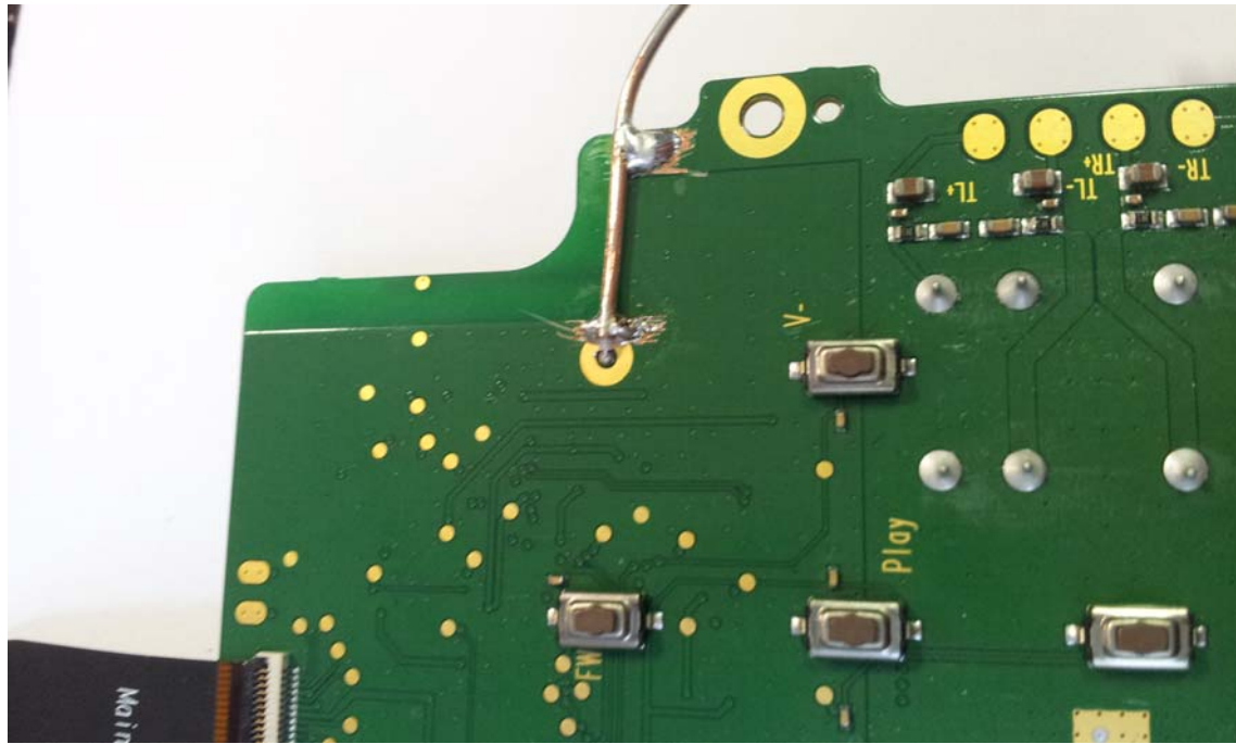
Bluetooth radio backside from conducted sample
