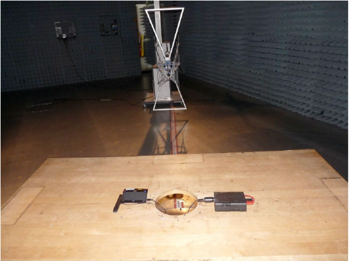
Photo 2: Test setup for radiated measurements (Enclosure, 30 MHz –1 GHz) EUT powered by: DC/DC converter
