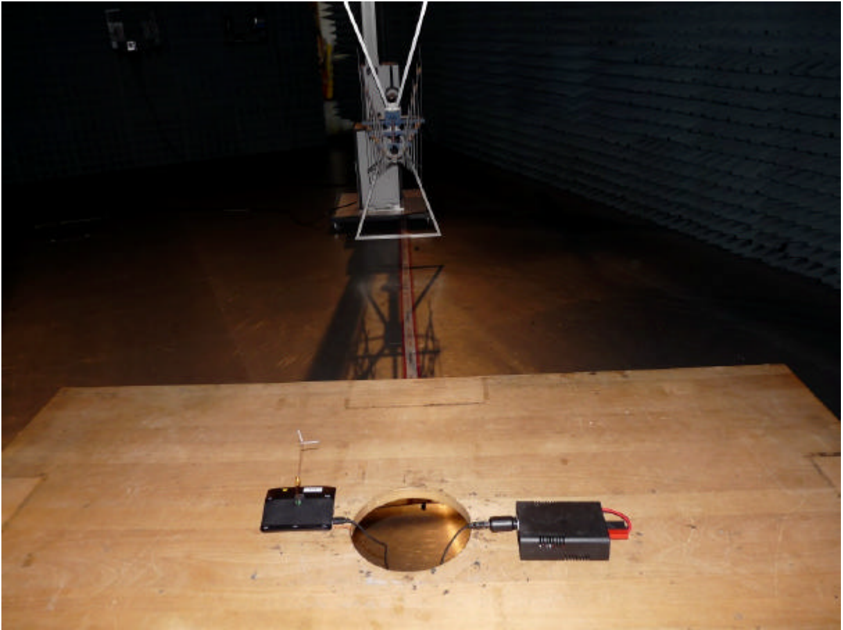
Photo 3: Test setup for radiated measurements (Enclosure, 30 MHz –1 GHz) EUT powered by: AC/DC converter
