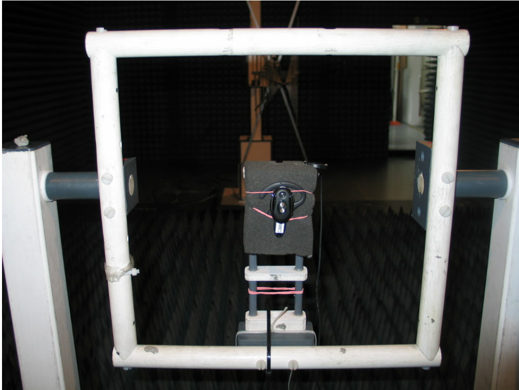
Photo 3: Test setup for radiated measurements
