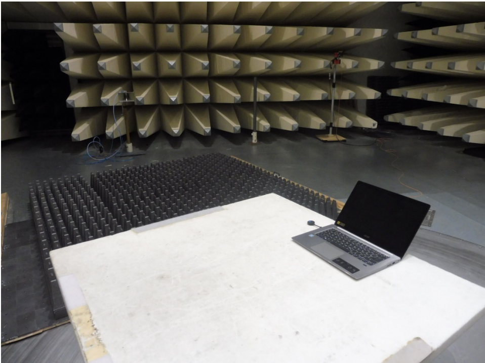
Photo 2: Radiated Emission
