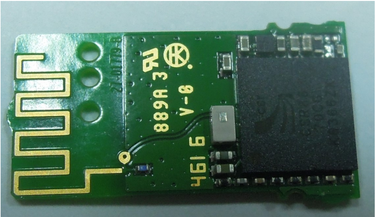
Internal photos of Link 370
