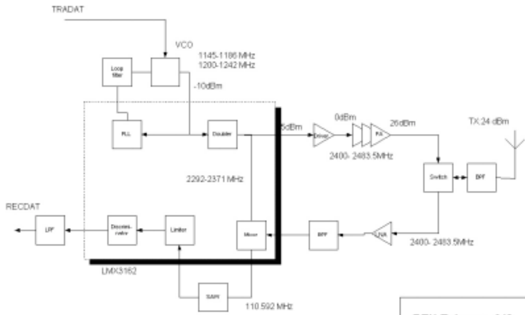
RTX Telecom A/S MARS RF Block diagram
