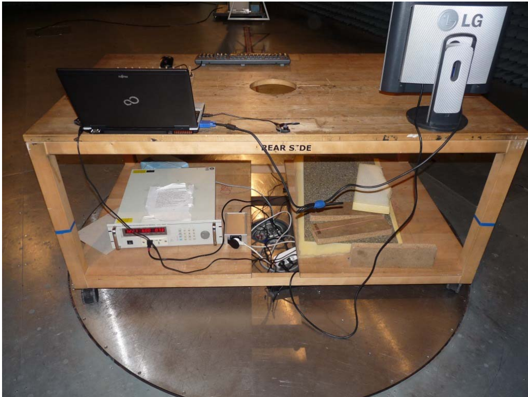
Photo 4: Test setup for radiated measurements (computer peripheral setup, EUT supplied by USB-cable from computer, unintentional radiator S15)
