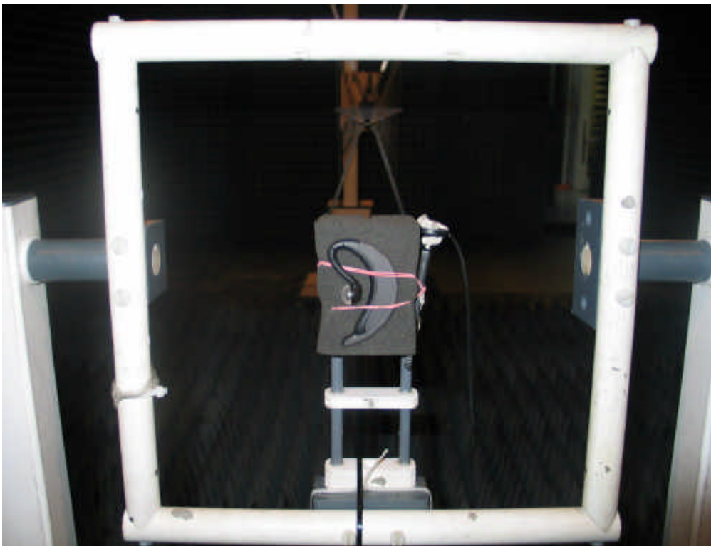
Photo 2: Test setup for radiated measurements (Enclosure, above 1 GHz)
