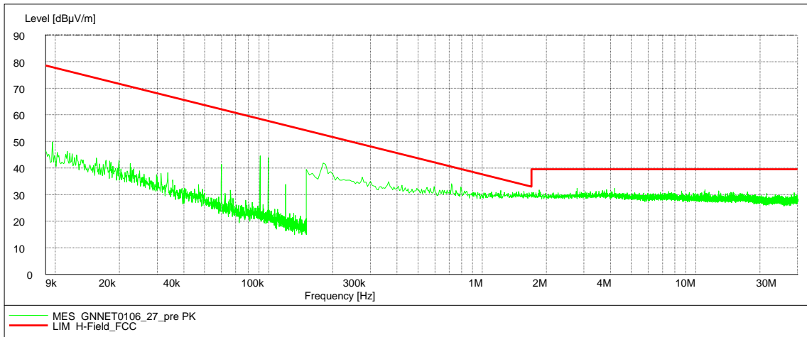
Antenna position 0° EUT position front side
