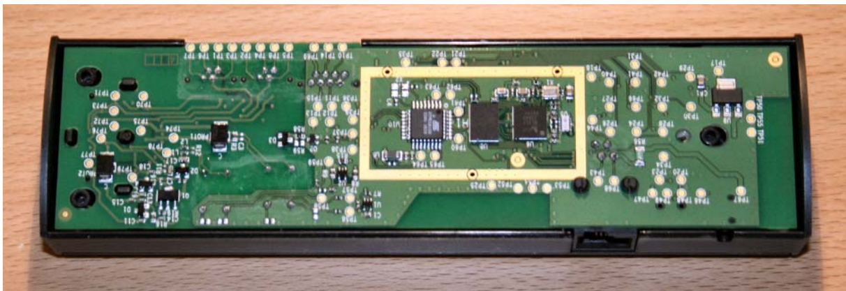
Figur 5: A7010 PCB bottom side
