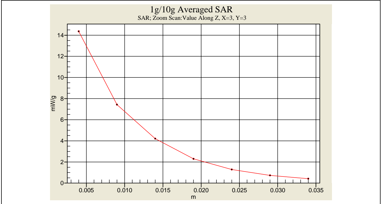
Body-Tissue-Simulating-Liquid 2.4GHz
