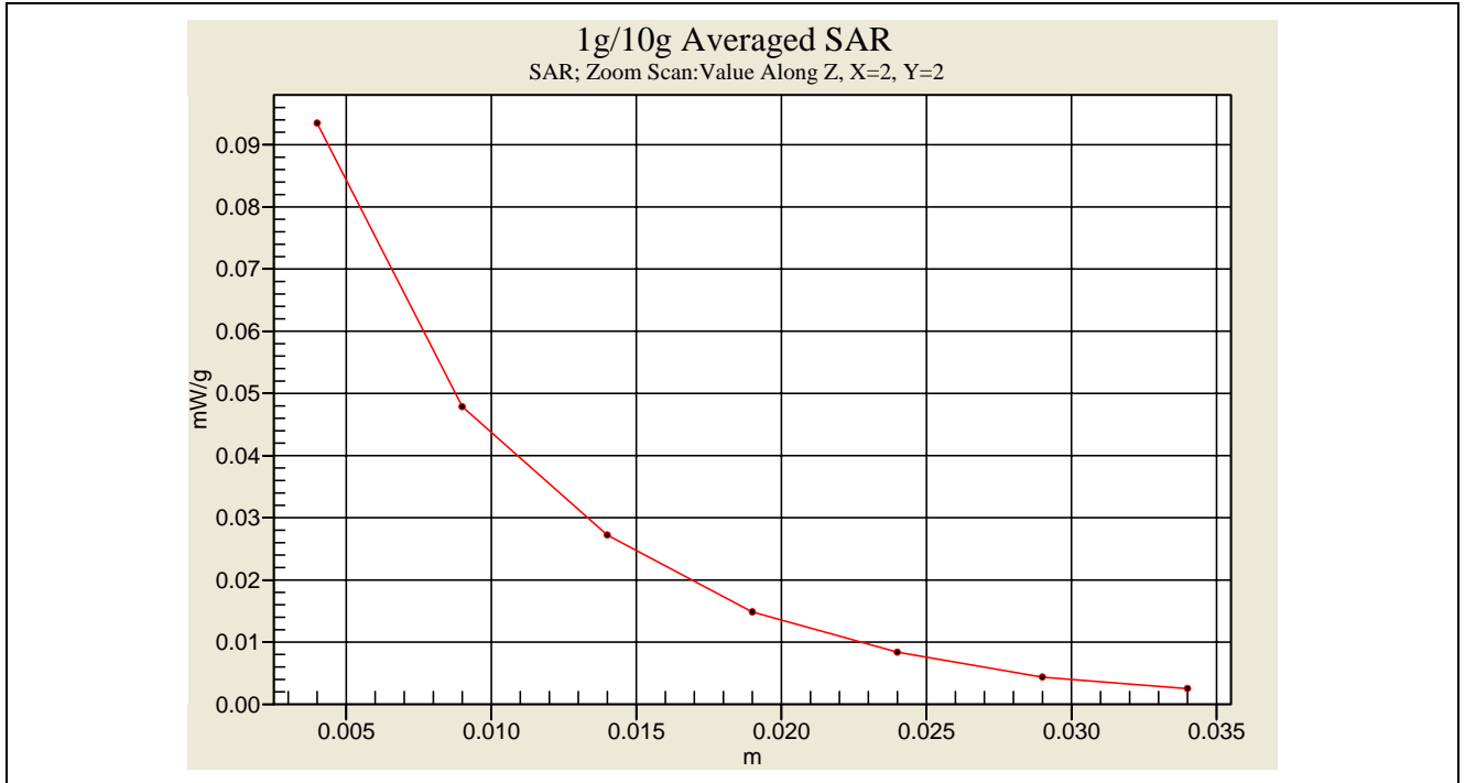
SAR Measurement _ Flat Bluetooth CH78
