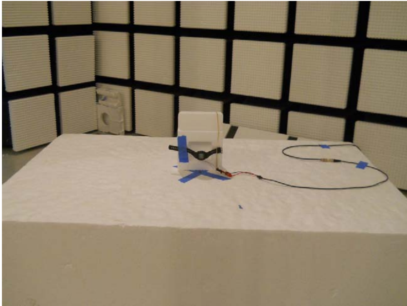
RADIATED BELOW 1GHz FRONT PHOTO
