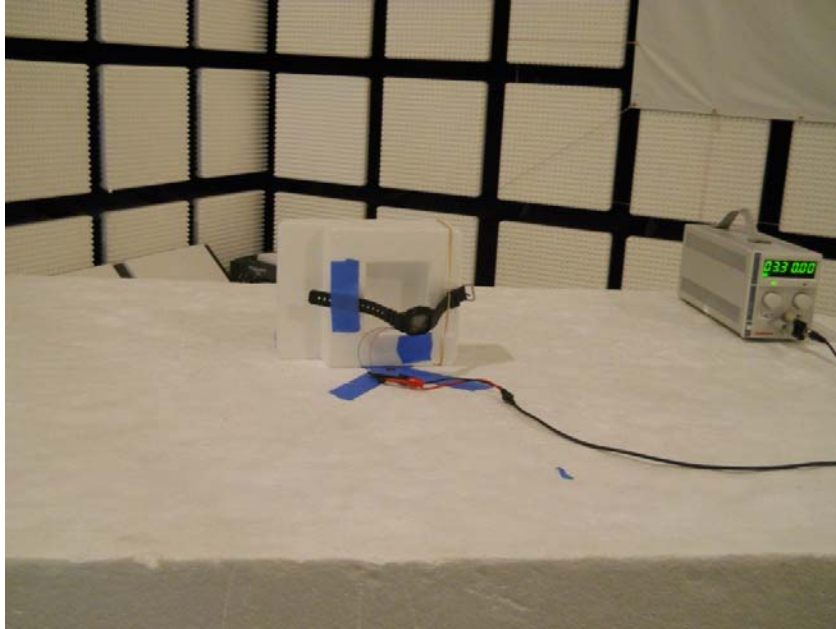
RADIATED ABOVE 1GHz FRONT PHOTO
