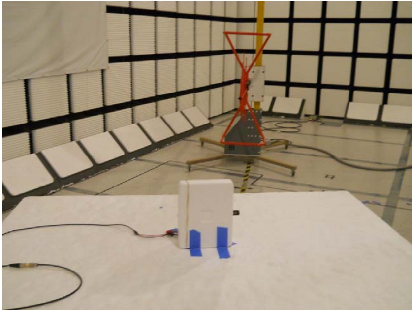
RADIATED BELOW 1GHz REAR PHOTO
