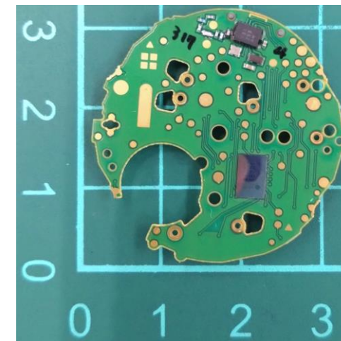
RF Module In Watch Module
