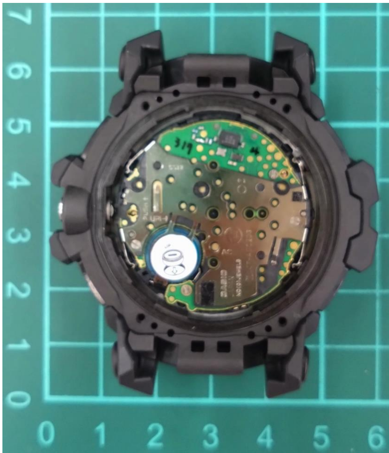
Module in Watch case
