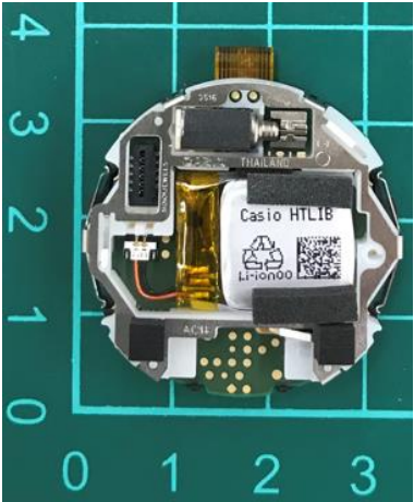
Watch Module Back side
