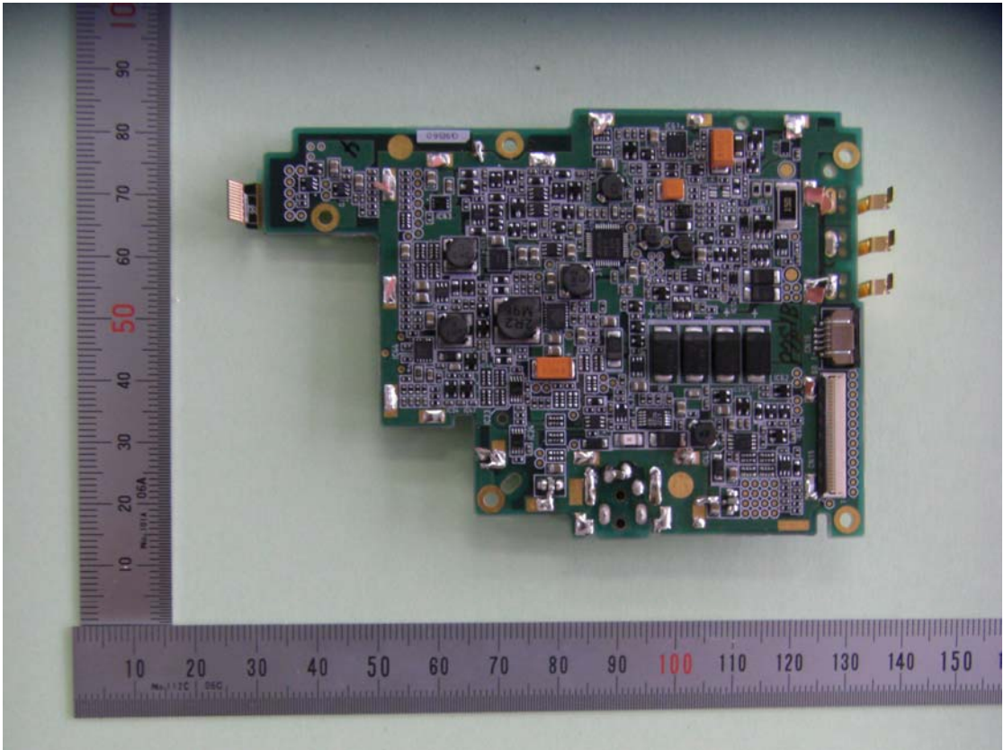
2D Scanner
