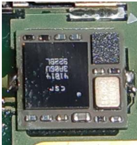
Bluetooth module without Shield cover
