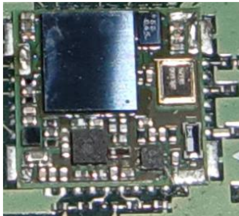
WLAN module without Shield cover
