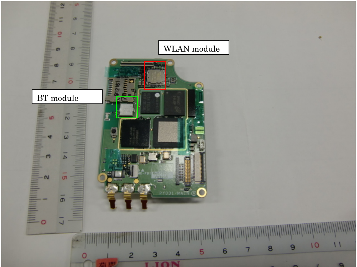
WLAN module without Shield cover
