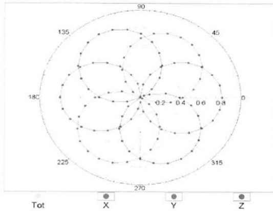
f=600 MHz,TEM
