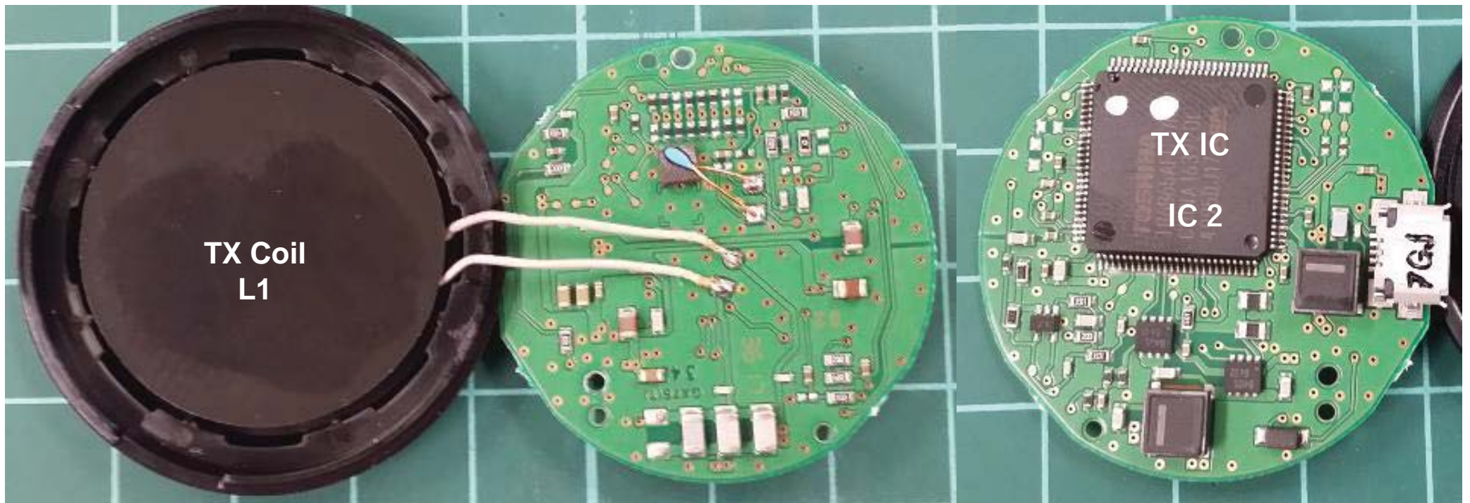
Front side
