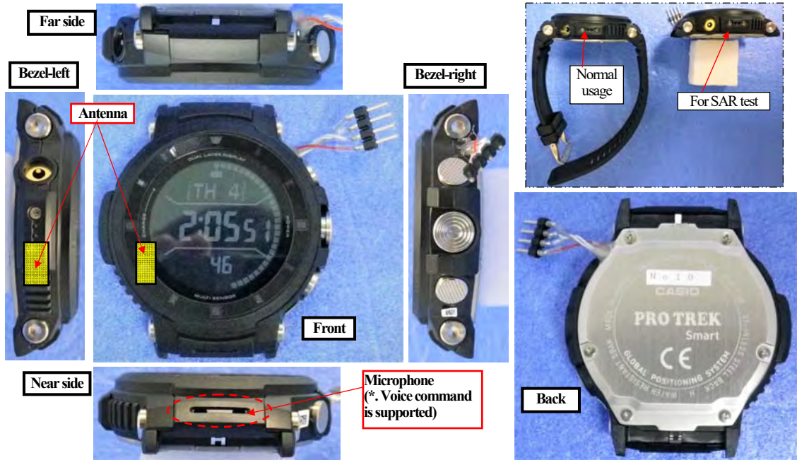
Antenna location and antenna distance [Unit: mm]
