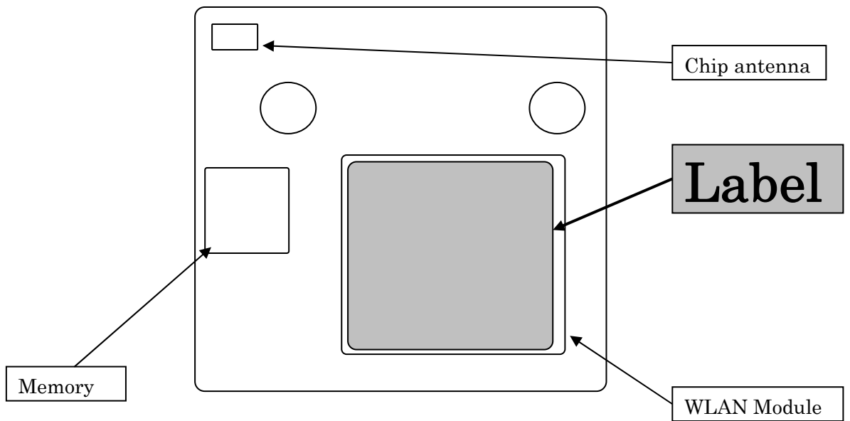
Fig.1 IC side view
