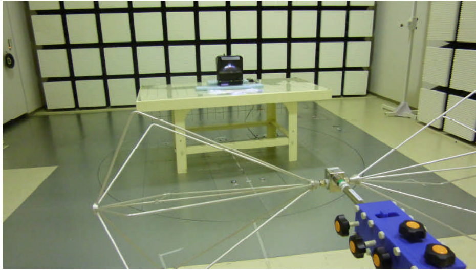
Photo3 Test setup for Radiated ( above 30MHz )
