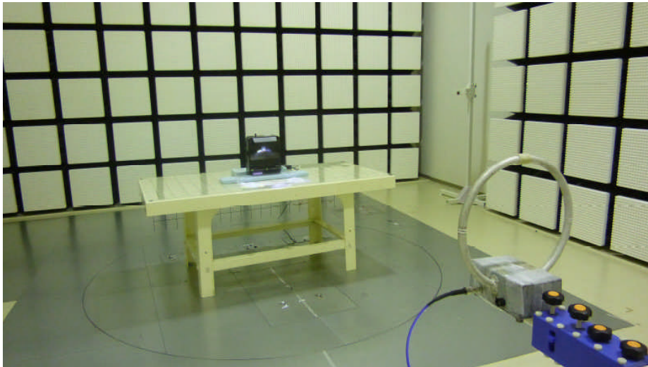
Photo2 Test setup for Radiated ( below 30MHz )
