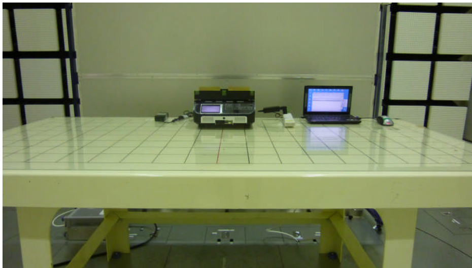
Photo4 Test Setup for Conducted Test_1 (Front)
