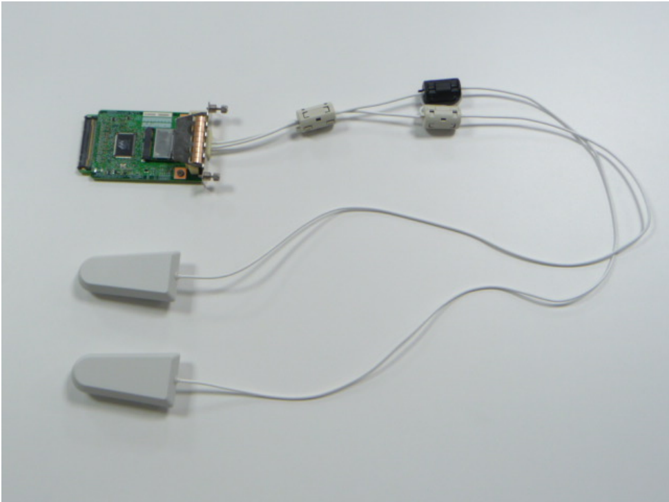
Module with Dipole Antenna (Top)
