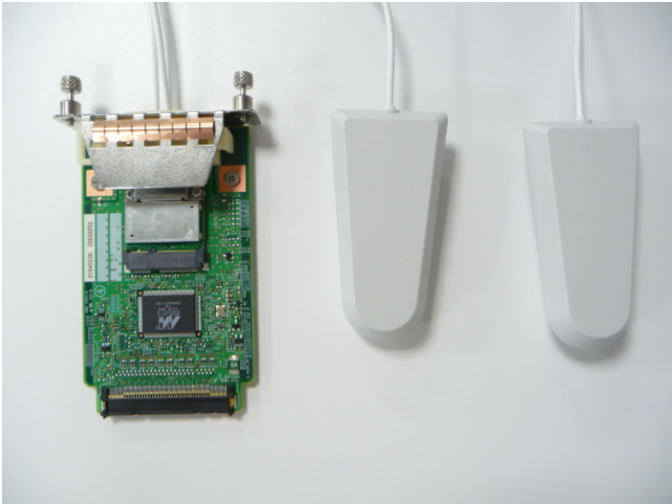
Module with Dipole Antenna (Top) [Closeup]
