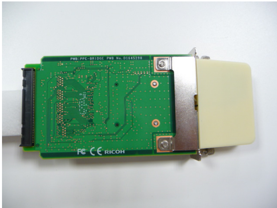
Module with Inverted F Antenna (Bottom)
