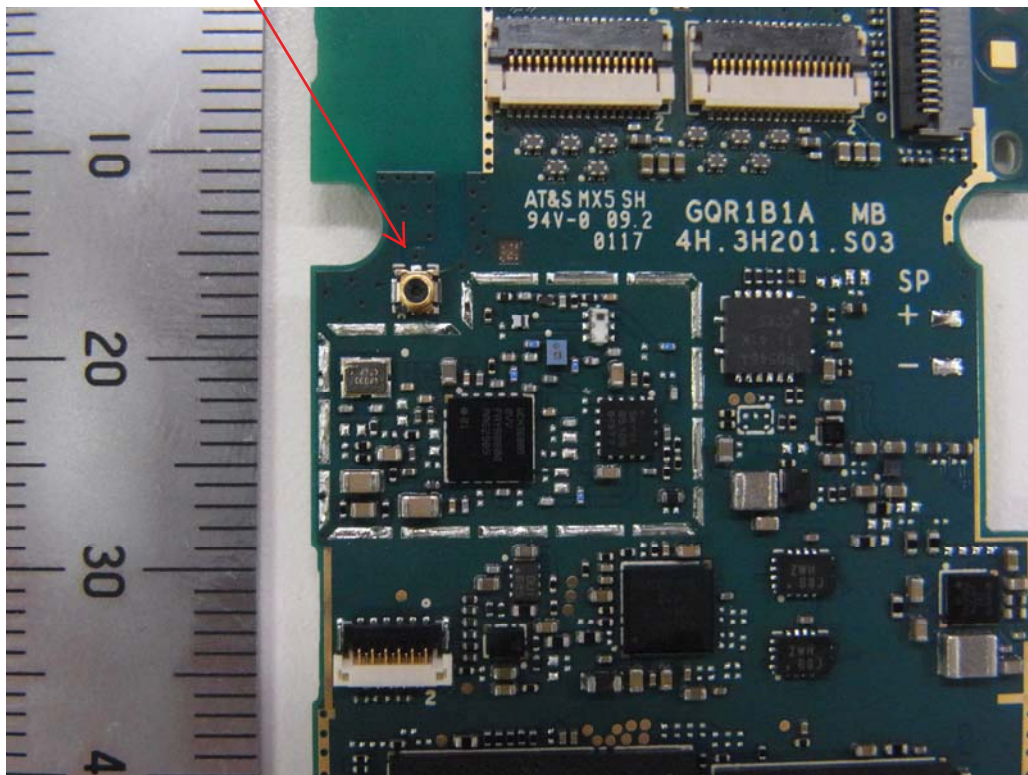
MAIN_top_RF_Expansion
