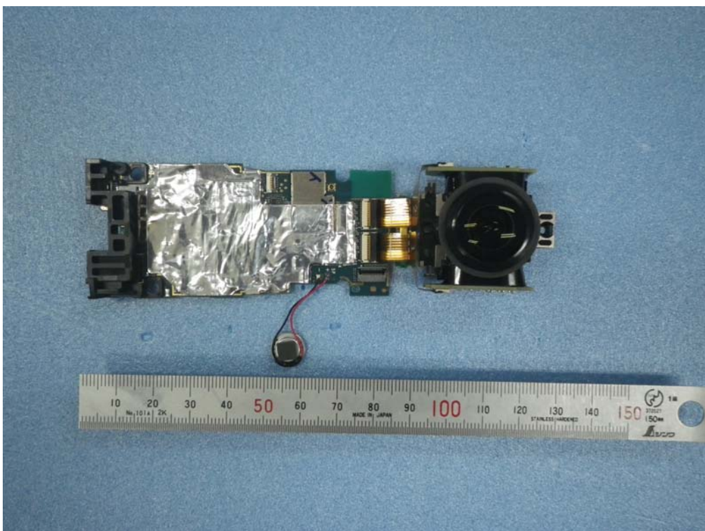
Lens Main PCB Front Side
