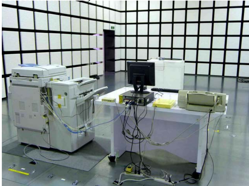
Loop antenna horizontal view
