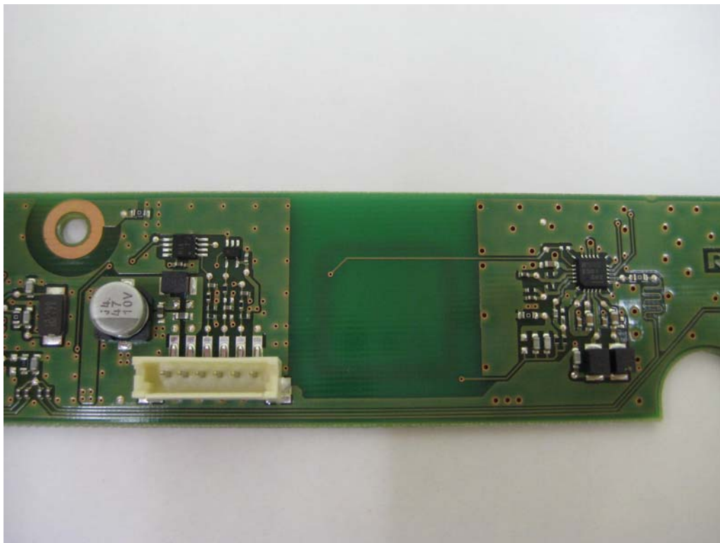
RFID Module Front (Enlarged) - Center Right
