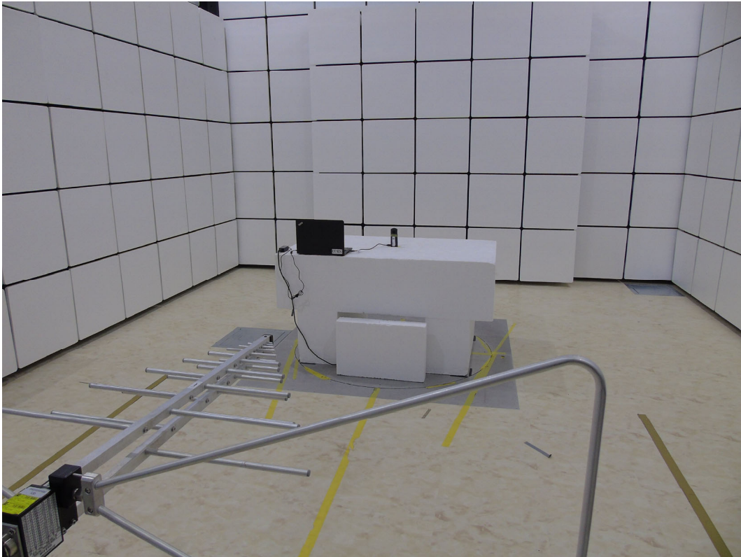
Radiated Test
