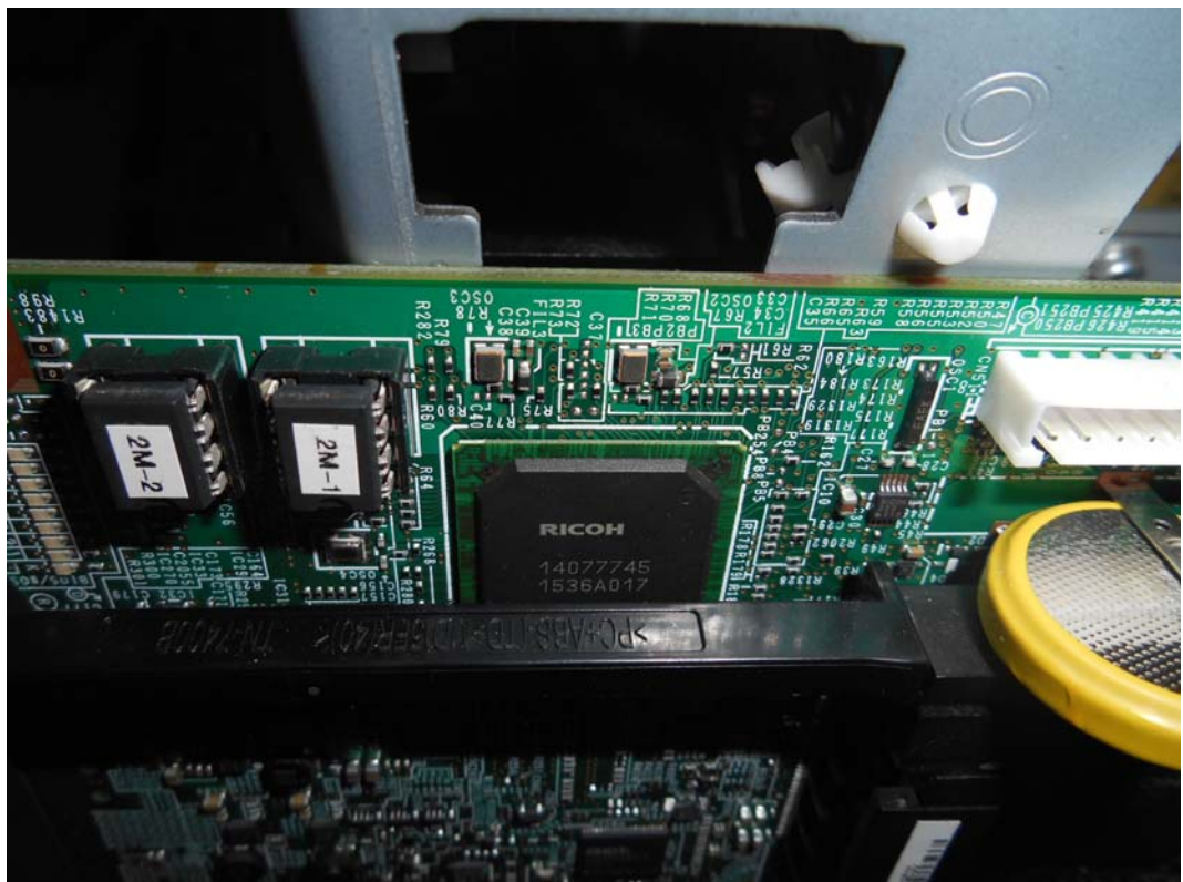
FIGURE 39 PRINTER (M/N: SP C342DN ) CHIP#2 AND CRYSTAL#2 ON MAIN BOARD
