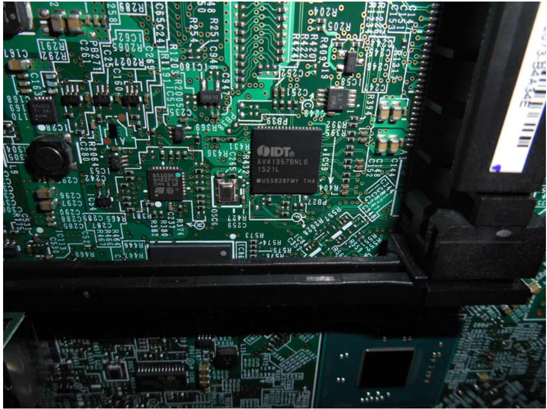
FIGURE 80 PRINTER (M/N: SP C340DN ) CHIP#2 AND CRYSTAL#2 ON MAIN BOARD
