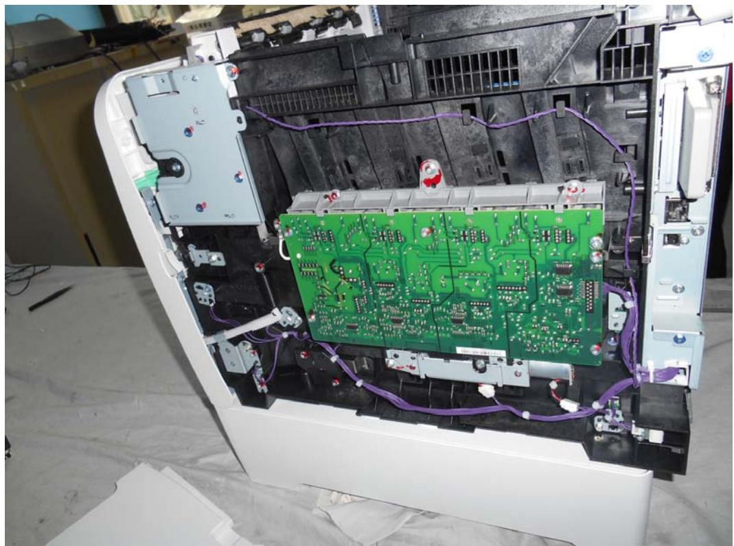
FIGURE 27 PRINTER (M/N: SP C342DN) SIDE#2 COVER REMOVED
