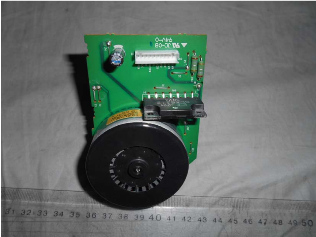
FIGURE 19 PRINTER (M/N: SP C342DN ) MOTOR BOARD#2 (COMPONENT SIDE)
