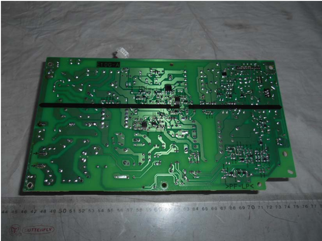
FIGURE 11 PRINTER (M/N: SP C342DN) POWER BOARD (SOLDERED SIDE)
