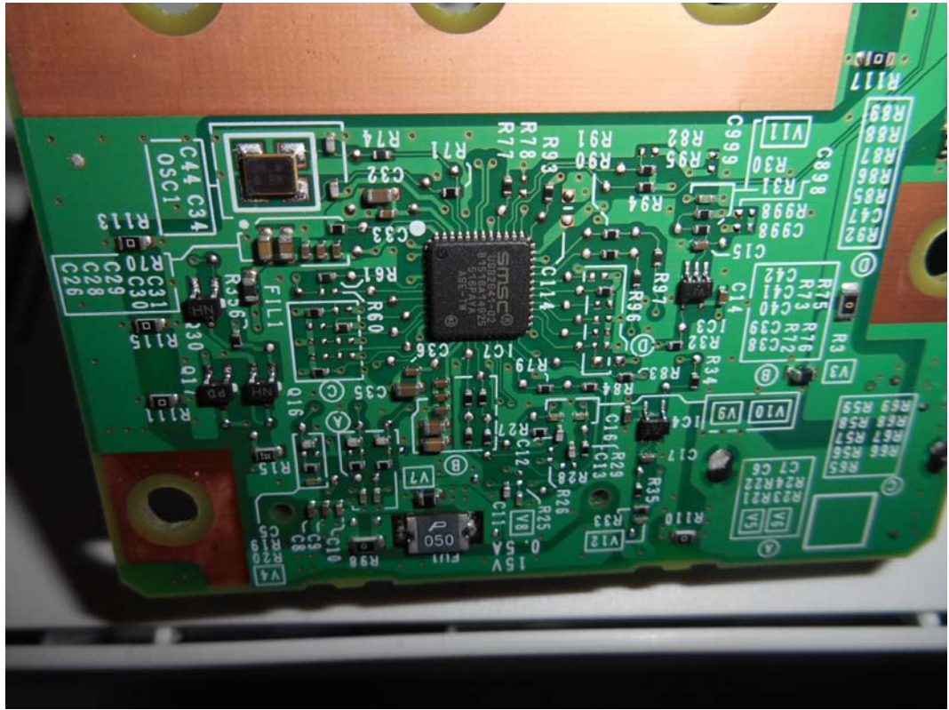
FIGURE 4 PRINTER (M/N: SP C342DN) CHIP#1 AND CRYSTAL#1 ON CONTROL BOARD
