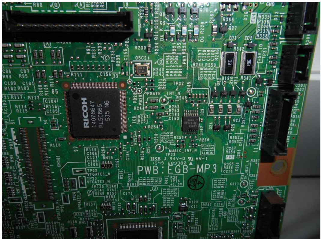
FIGURE 33 PRINTER (M/N: SP C342DN) CHIP#1 AND CRYSTAL#1 ON MAIN BOARD
