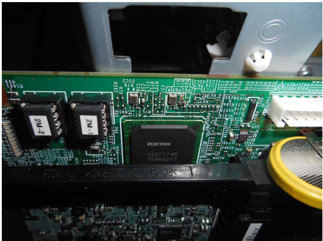
FIGURE 81 PRINTER (M/N: SP C340DN ) CHIP#2 AND CRYSTAL#2 ON MAIN BOARD
