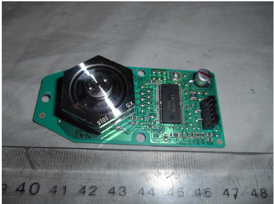
FIGURE 42 PRINTER (M/N: SP C342DN ) BOARD #3 (COMPONENT SIDE)
