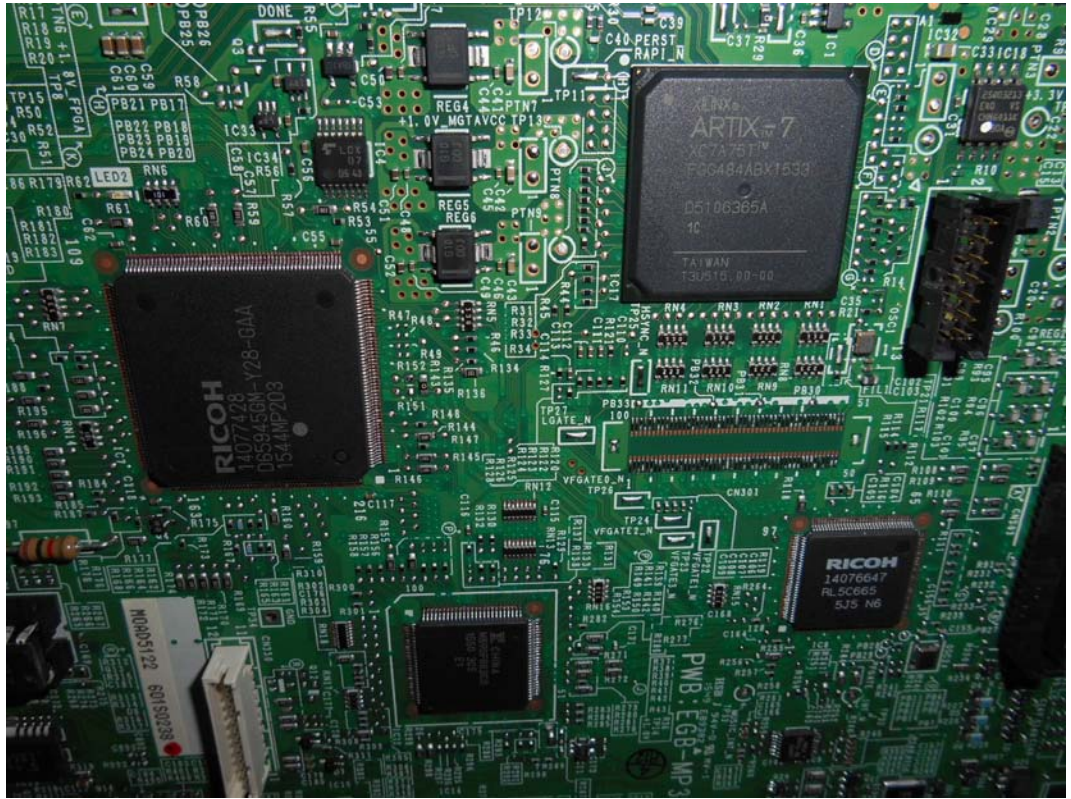
FIGURE 76 PRINTER (M/N: SP C340DN ) CHIP#1 AND CRYSTAL#1 ON MAIN BOARD
