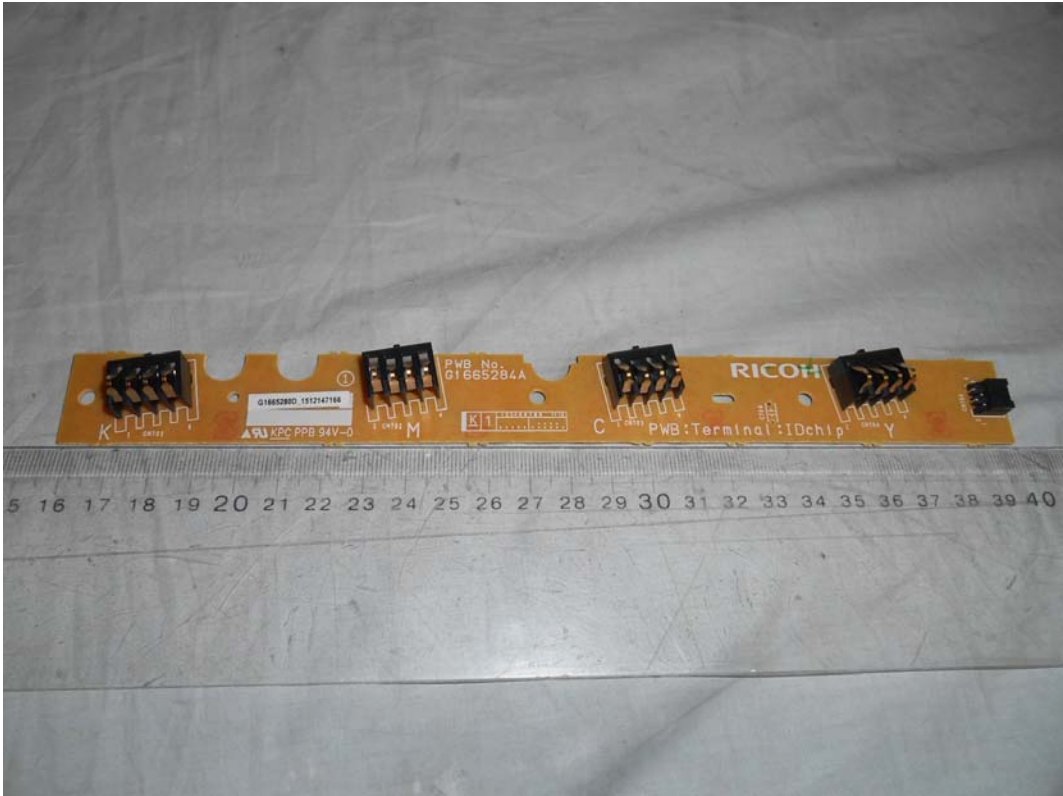
FIGURE 25 PRINTER (M/N: SP C342DN) BOARD#1 (COMPONENT SIDE)
