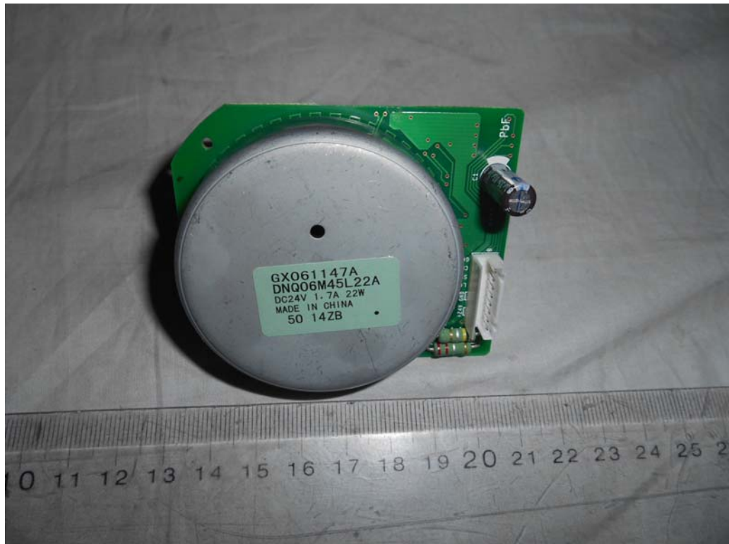
FIGURE 58 PRINTER (M/N: SP C340DN ) MOTOR BOARD#1 (COMPONENT SIDE)
