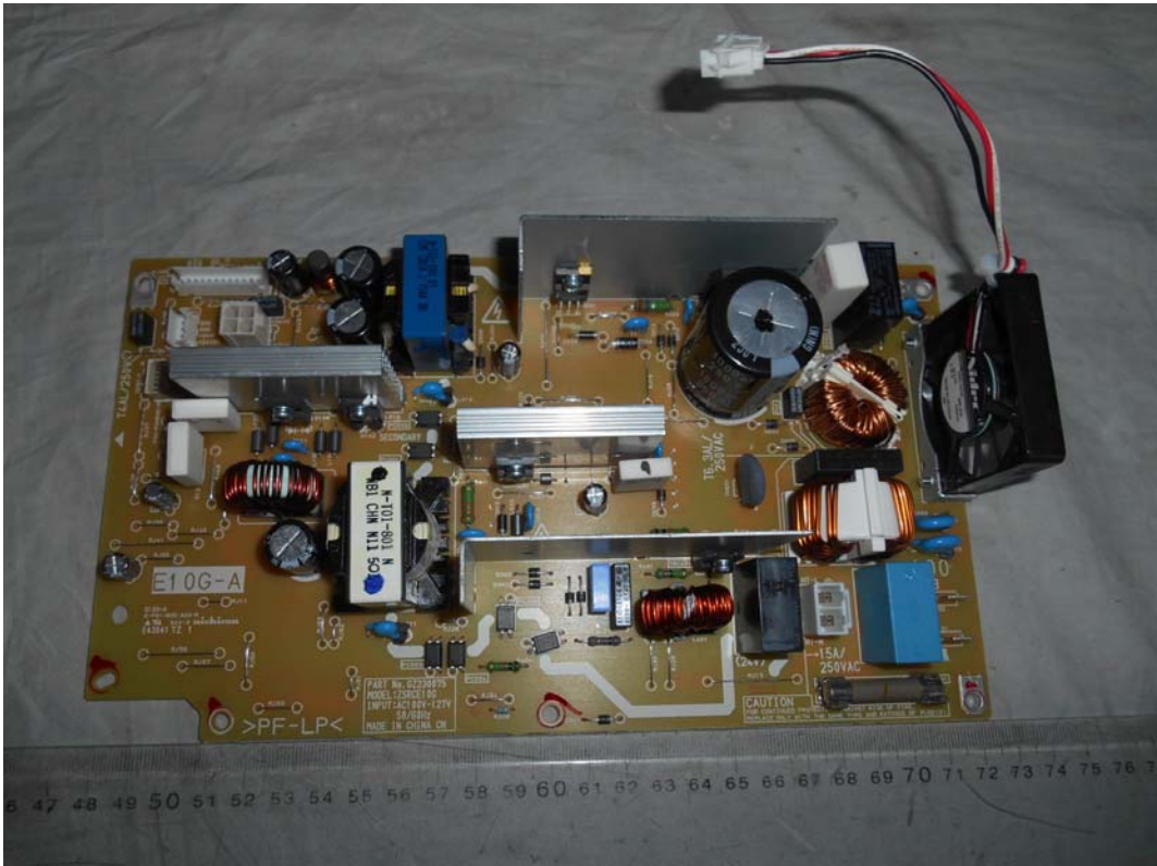
FIGURE 10 PRINTER (M/N: SP C342DN) POWER BOARD (COMPONENT SIDE)
