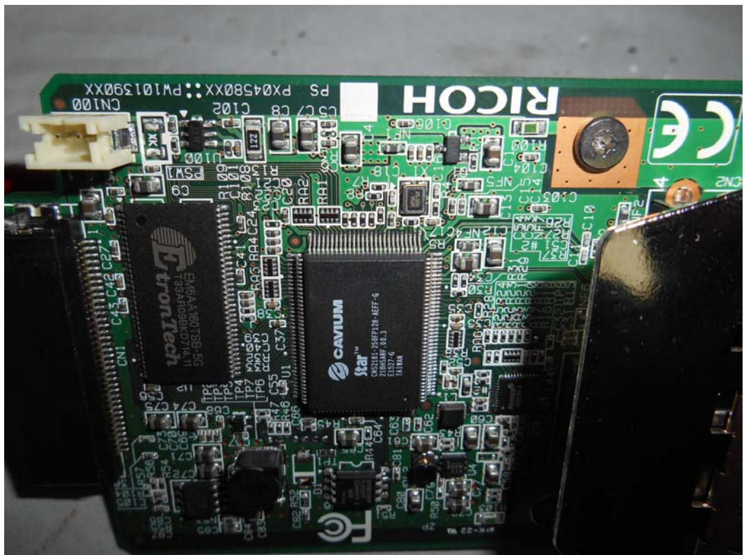
FIGURE 91 PRINTER (M/N: SP C342DN SP C340DN ) CHIP AND CRYSTAL ON NIC2 BOARD
