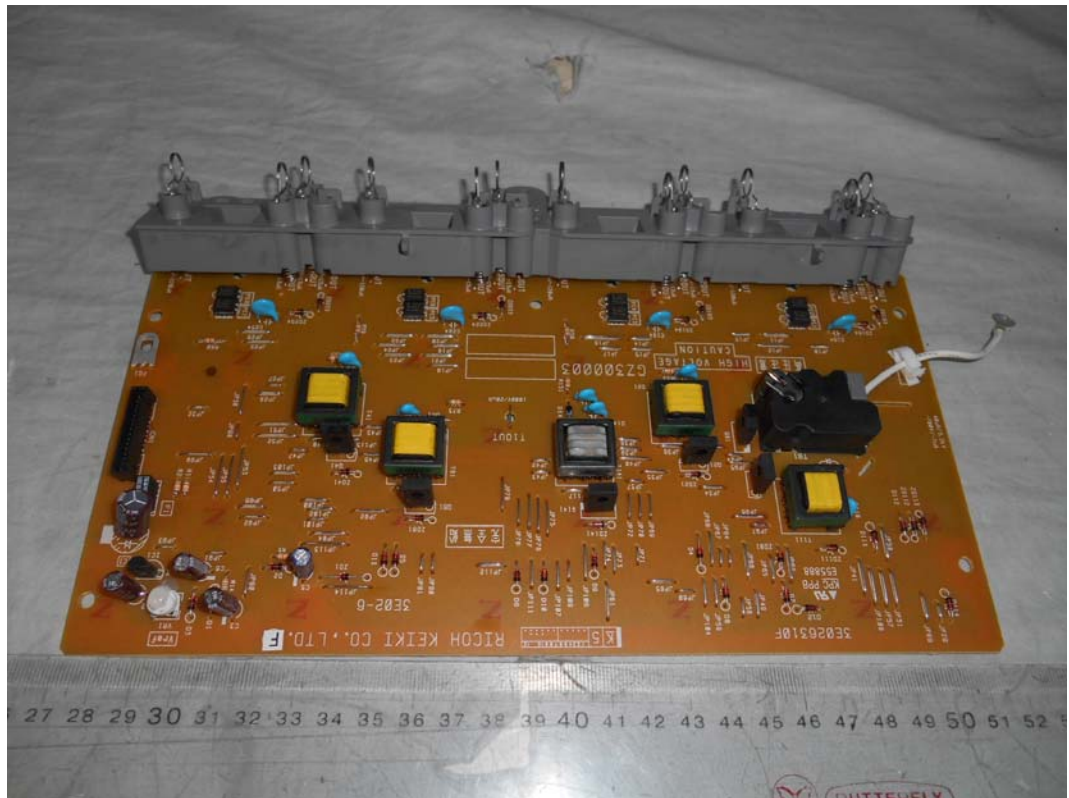
FIGURE 28 PRINTER (M/N: SP C342DN ) BOARD #2 (COMPONENT SIDE)
