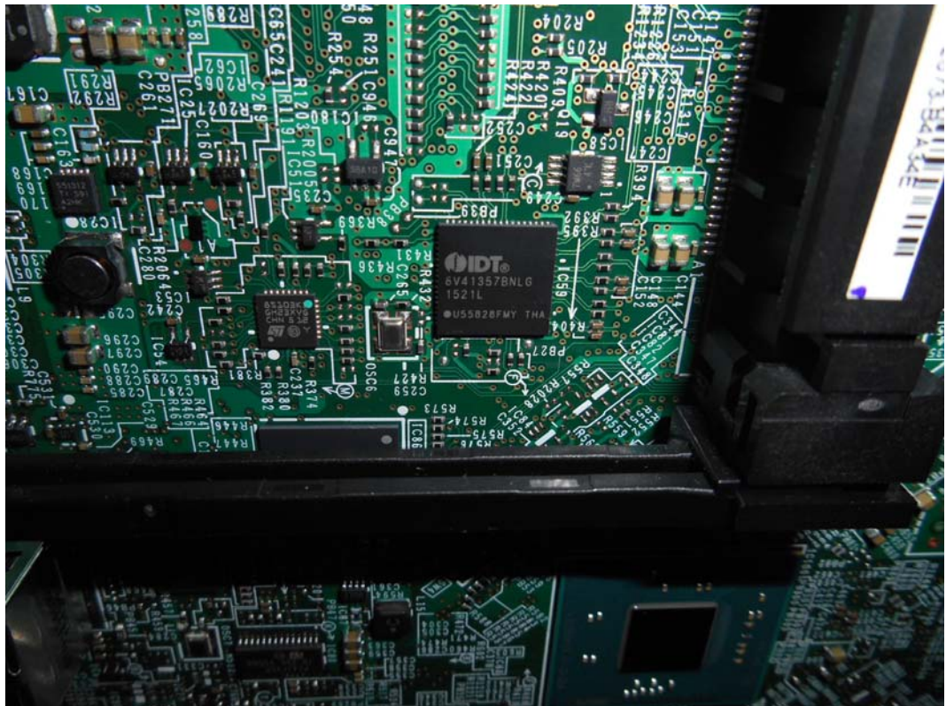
FIGURE 38 PRINTER (M/N: SP C342DN ) CHIP#2 AND CRYSTAL#2 ON MAIN BOARD
