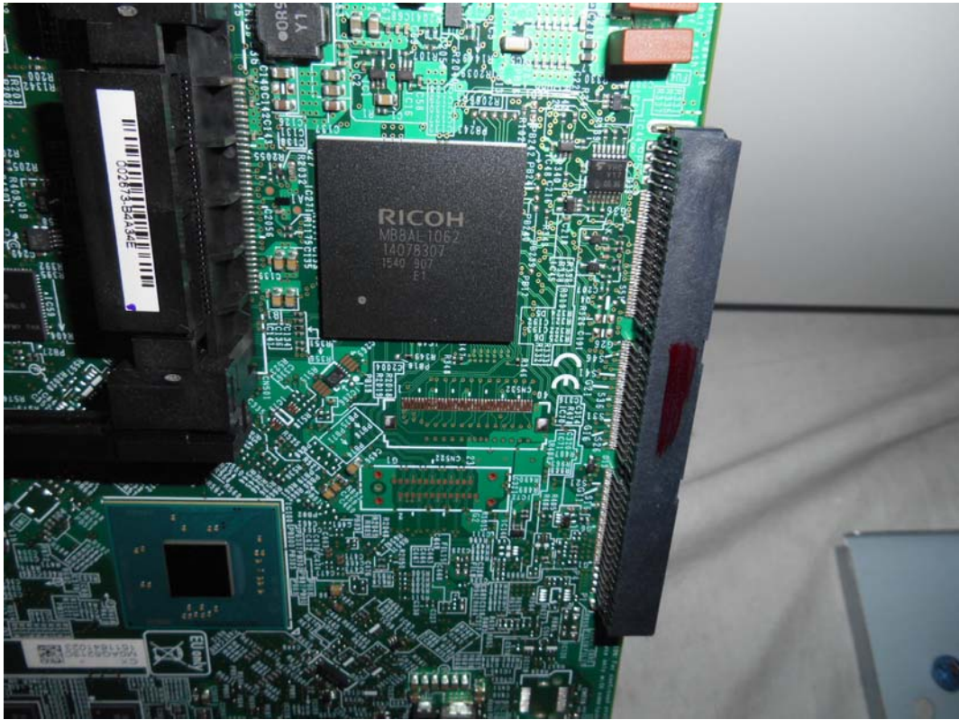
FIGURE 82 PRINTER (M/N: SP C340DN) CHIP#2 ON MAIN BOARD
