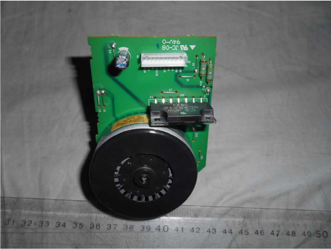
FIGURE 61 PRINTER (M/N: SP C340DN ) MOTOR BOARD#2 (COMPONENT SIDE)
