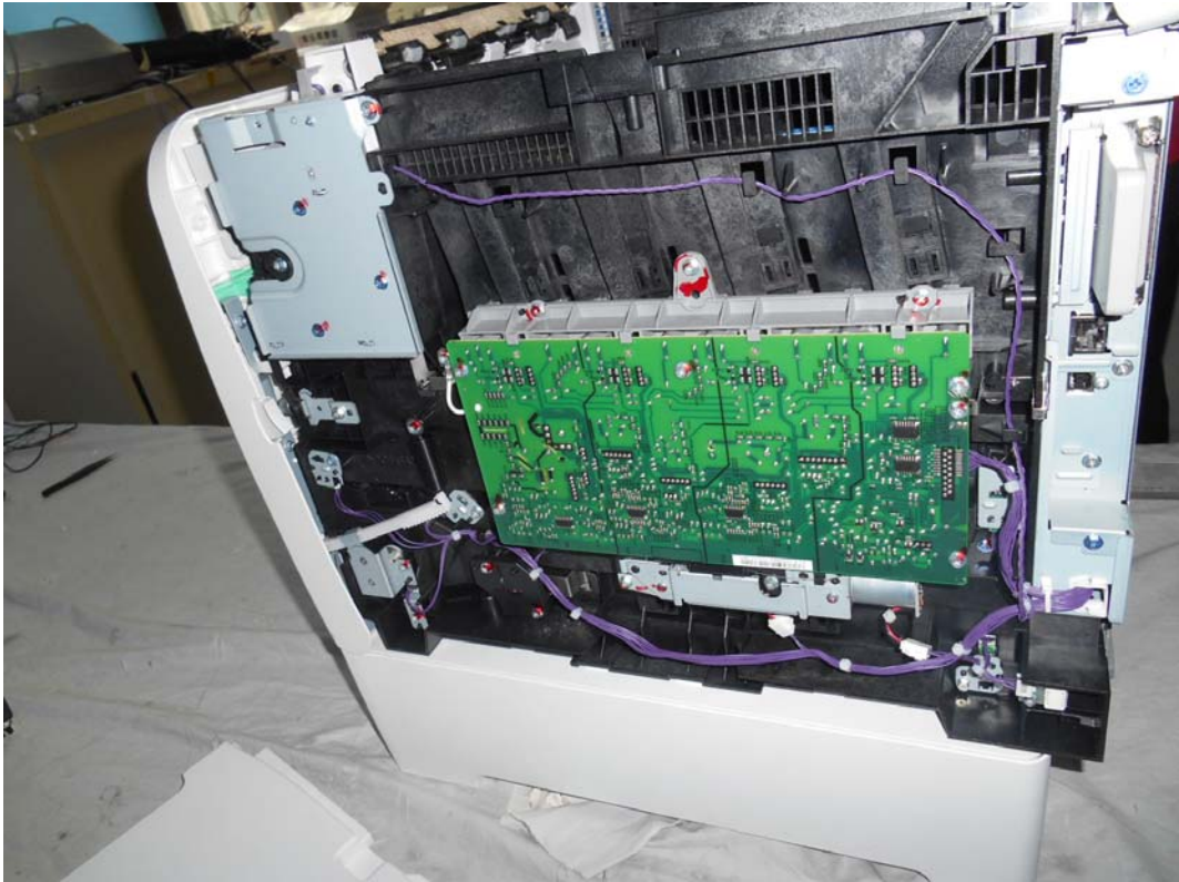
FIGURE 69 PRINTER (M/N: SP C340DN ) SIDE#2 COVER REMOVED
