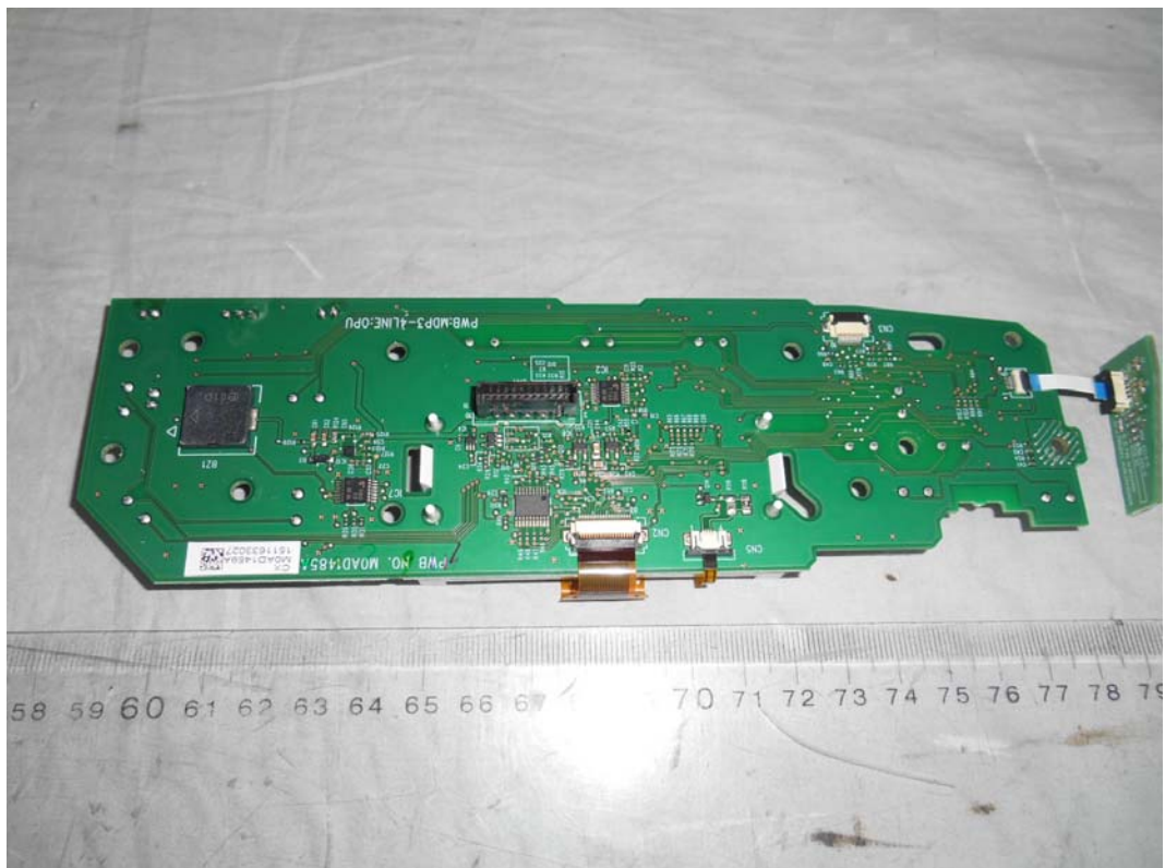
FIGURE 48 PRINTER (M/N: SP C340DN) CONTROL BOARD (SOLDERED SIDE)
