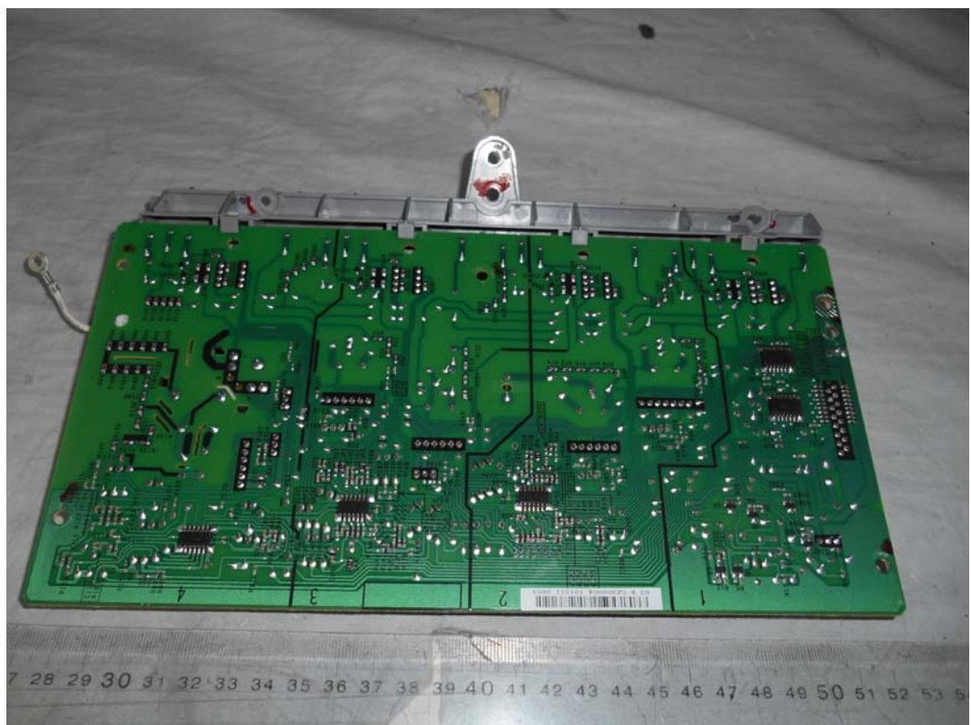
FIGURE 29 PRINTER (M/N: SP C342DN ) BOARD #2 (SOLDERED SIDE)
