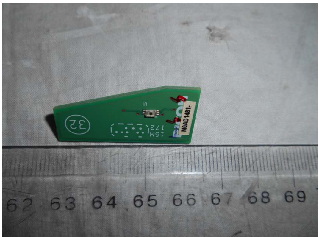
FIGURE 50 PRINTER (M/N: SP C340DN ) BOARD#1 (SOLDERED SIDE)
