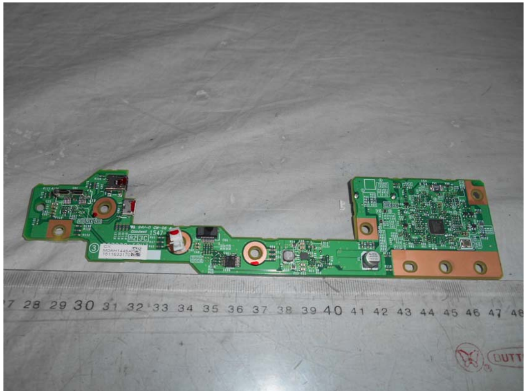
FIGURE 2 PRINTER (M/N: SP C342DN) CONTROL BOARD#1 (COMPONENT SIDE)
