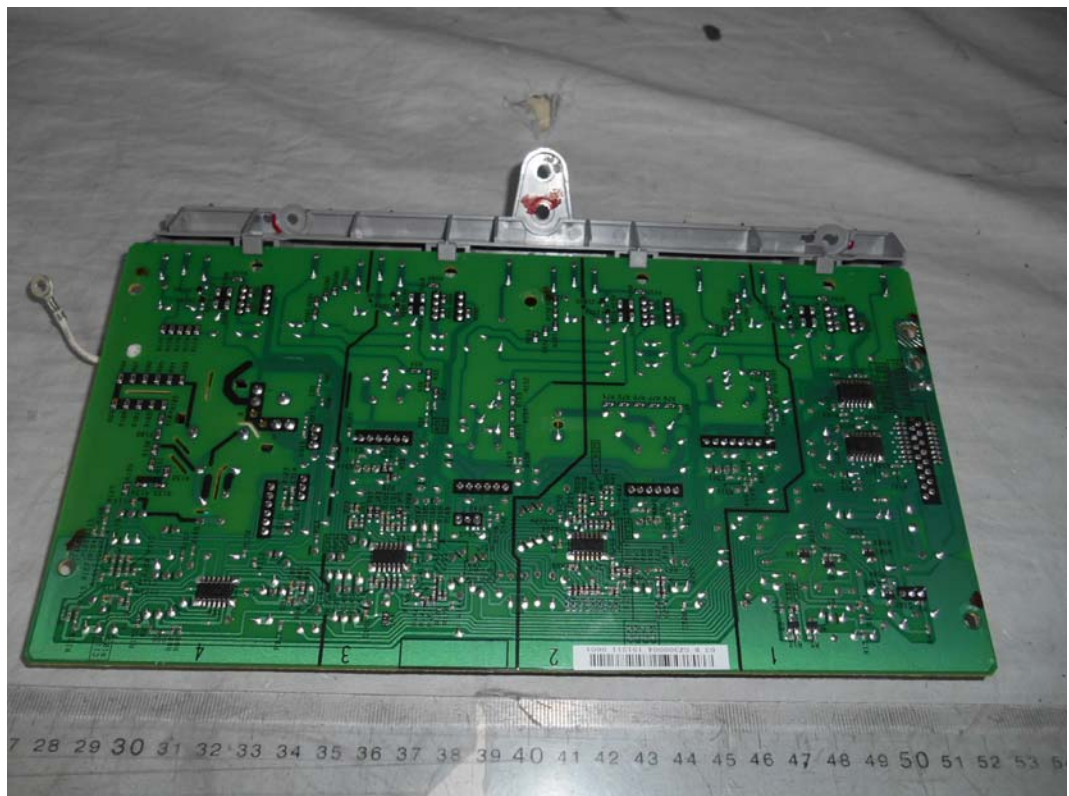
FIGURE 71 PRINTER (M/N: SP C340DN ) BOARD #3 (SOLDERED SIDE)
