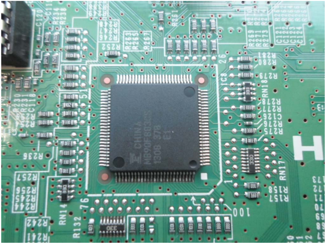
FIGURE 9 PRINTER (M/N: SP C252DN) CHIP #3 ON MAIN BOARD
