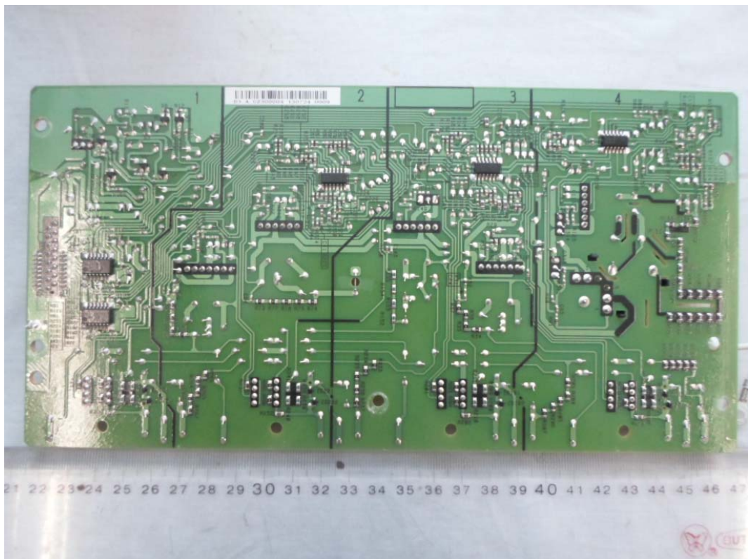
FIGURE 14 PRINTER (M/N: SP C252DN) POWER BOARD #2 (SOLDERED SIDE)
