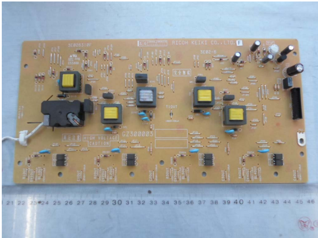
FIGURE 13 PRINTER (M/N: SP C252DN) POWER BOARD #2 (COMPONENT SIDE)
