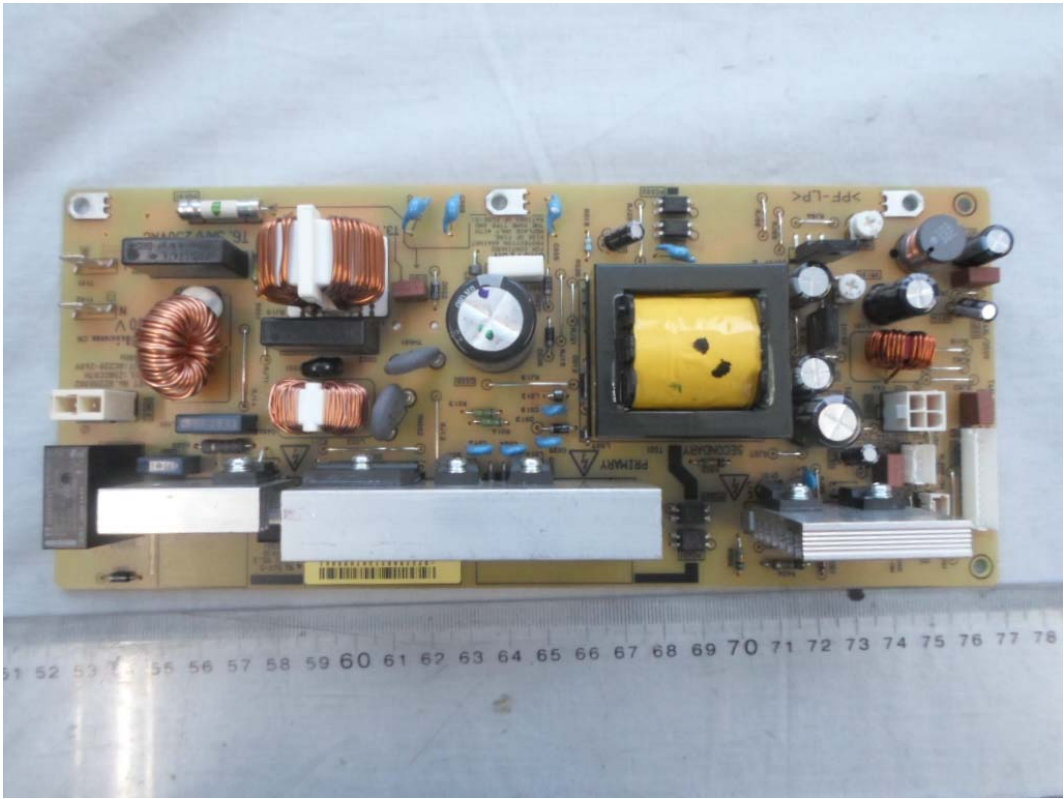
FIGURE 11 PRINTER (M/N: SP C252DN) POWER BOARD #1 (COMPONENT SIDE)
