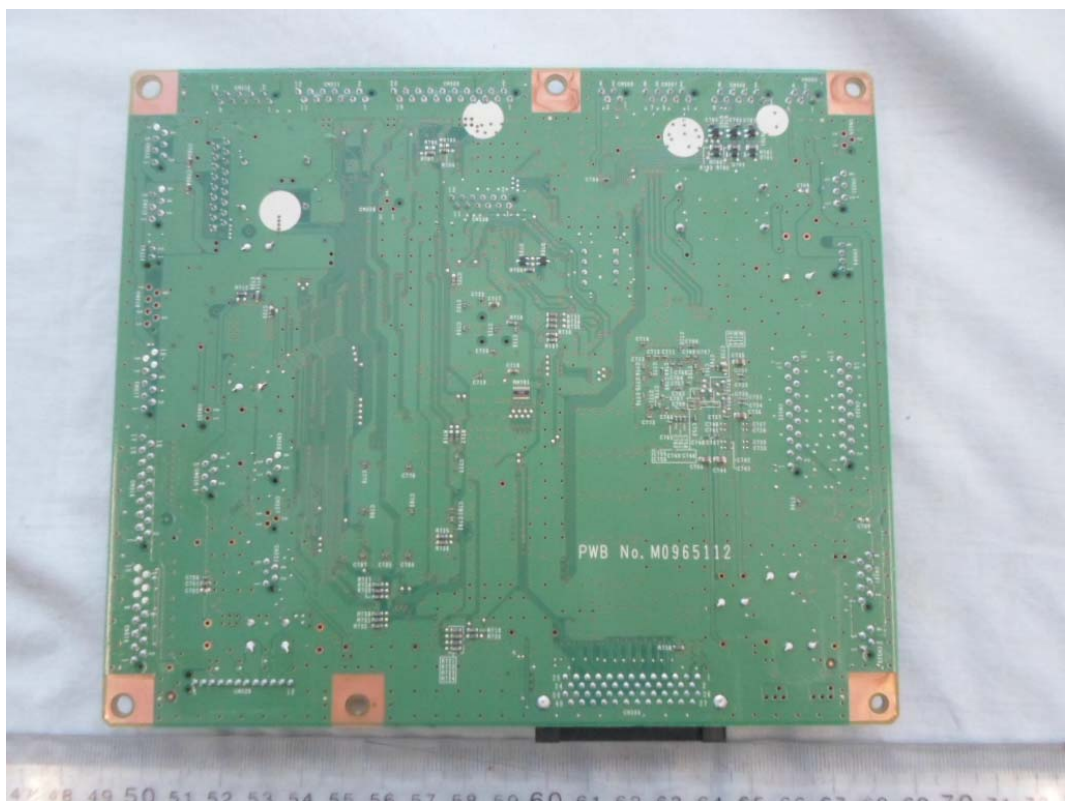
FIGURE 6 PRINTER (M/N: SP C252DN) MAIN BOARD (SOLDERED SIDE)
