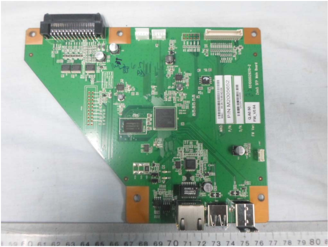
FIGURE 3 PRINTER (M/N: SP C252DN) SIGNAL BOARD (COMPONENT SIDE)
