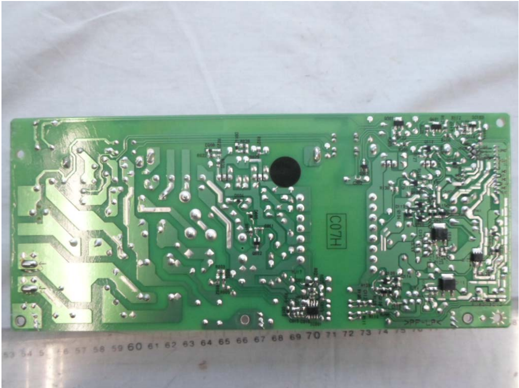
FIGURE 12 PRINTER (M/N: SP C252DN) POWER BOARD #1 (SOLDERED SIDE)
