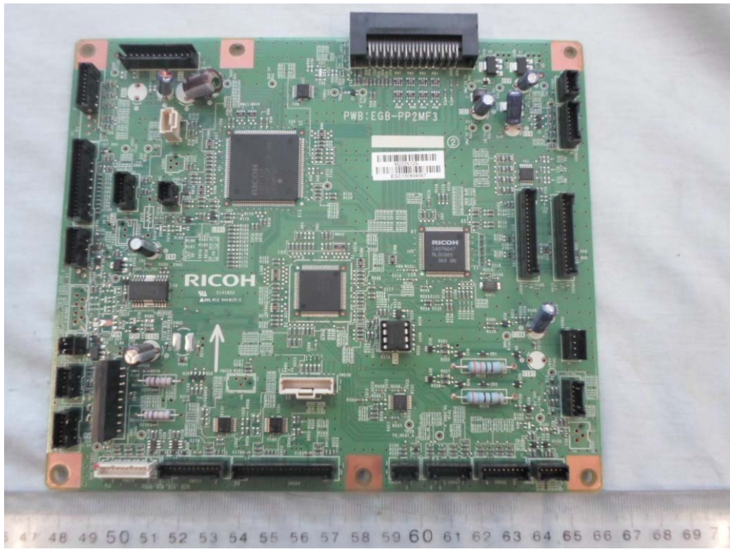
FIGURE 5 PRINTER (M/N: SP C252DN) MAIN BOARD (COMPONENT SIDE)
