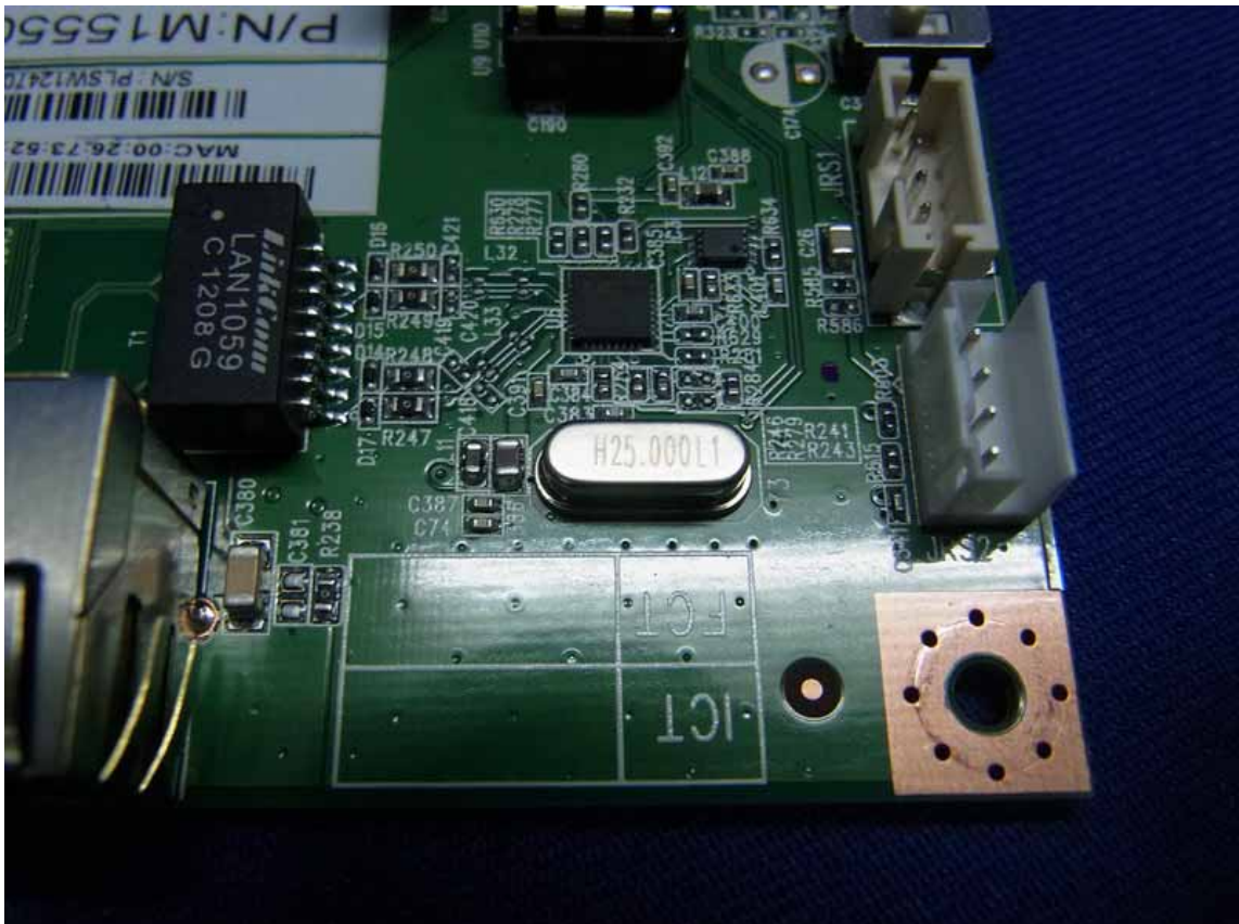
Figure 10 Frontside of the Main Board
