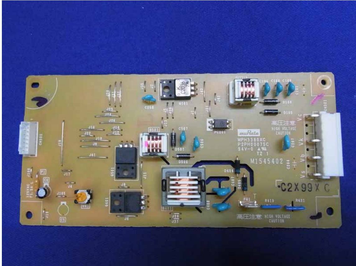
Figure 15 Frontside of the PCB
