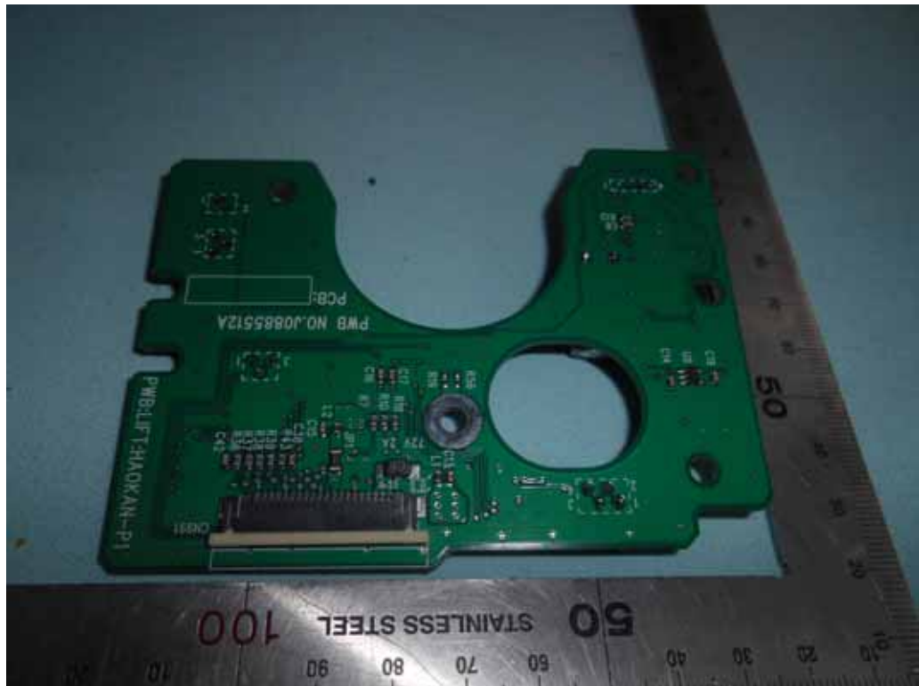
FIGURE 1 PRINTER (M/N: RICOH RI 100) BOARD#2 (SOLDERED SIDE)
