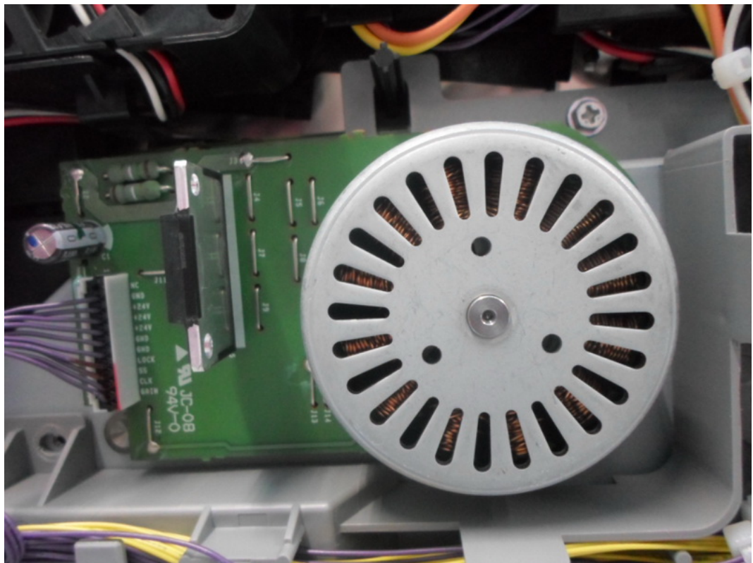
FIGURE 20 PRINTER (M/N: SP C262SFNw) MOTO #3
