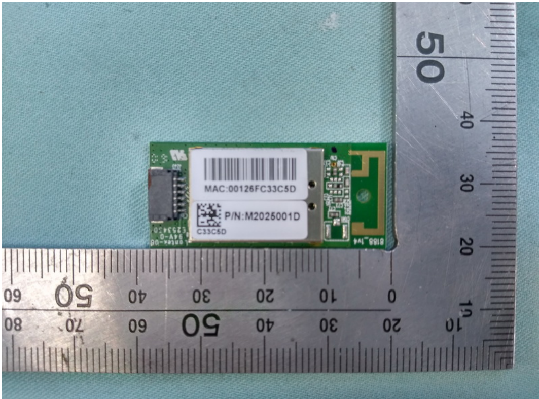
FIGURE 15 PRINTER (M/N: SP C262SFNW) WIFI BOARD (COMPONENT SIDE)
