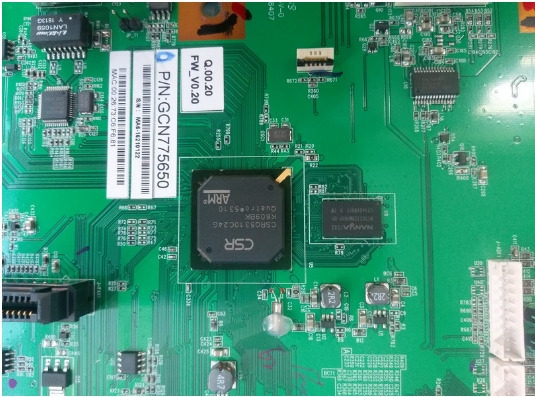
FIGURE 10 PRINTER (M/N: SP C262SFNW) CHIP AND CRYSTAL ON SIGNAL BOARD
