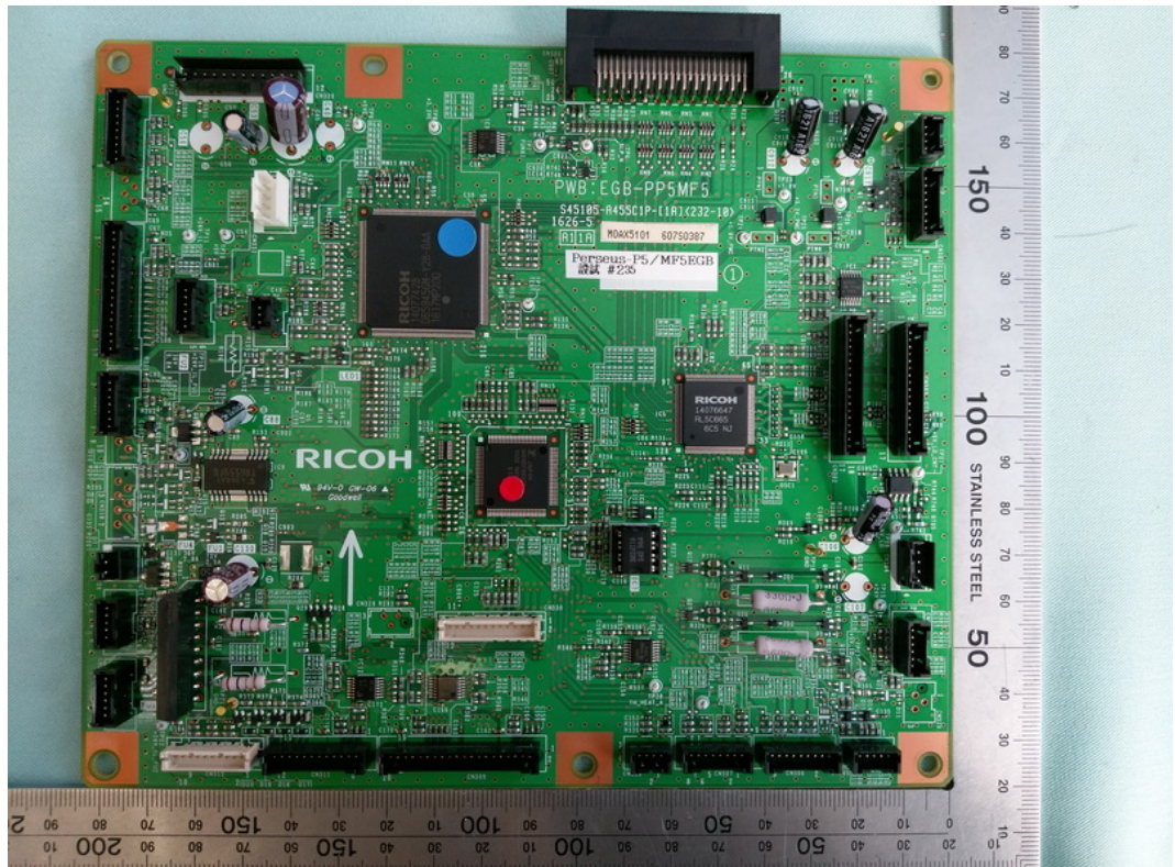
FIGURE 4 PRINTER (M/N: SP C262SFNW) MAIN BOARD (COMPONENT SIDE)
