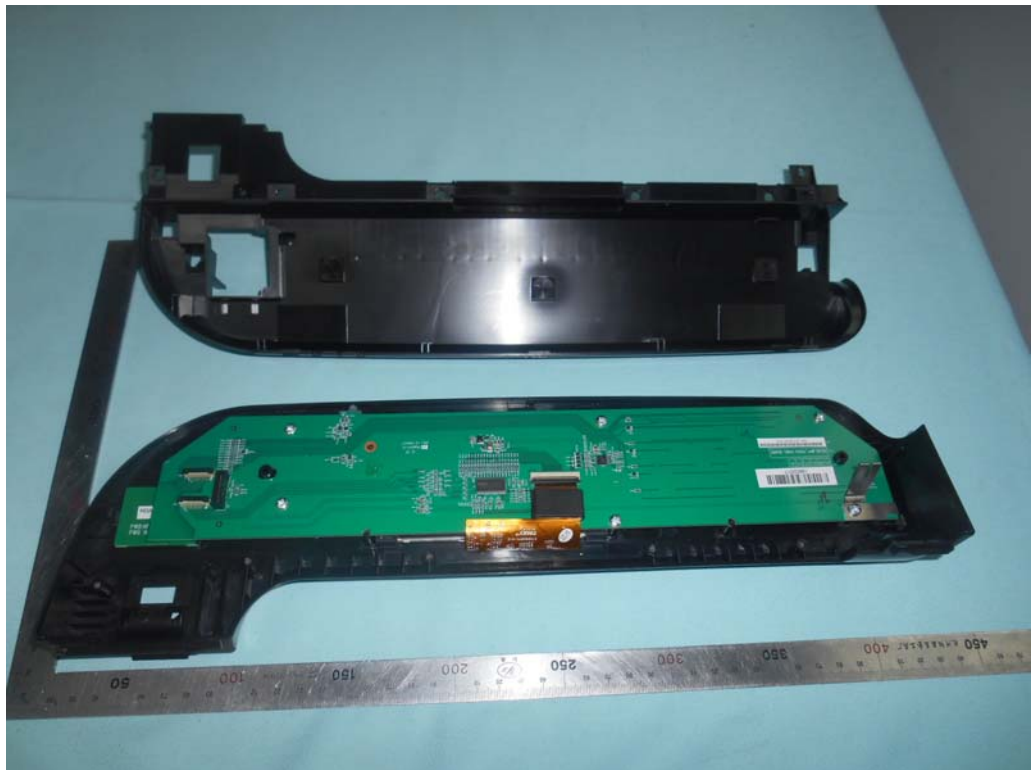
FIGURE 25 PRINTER (M/N: SP C262SFNW) PANEL COVER REMOVED
