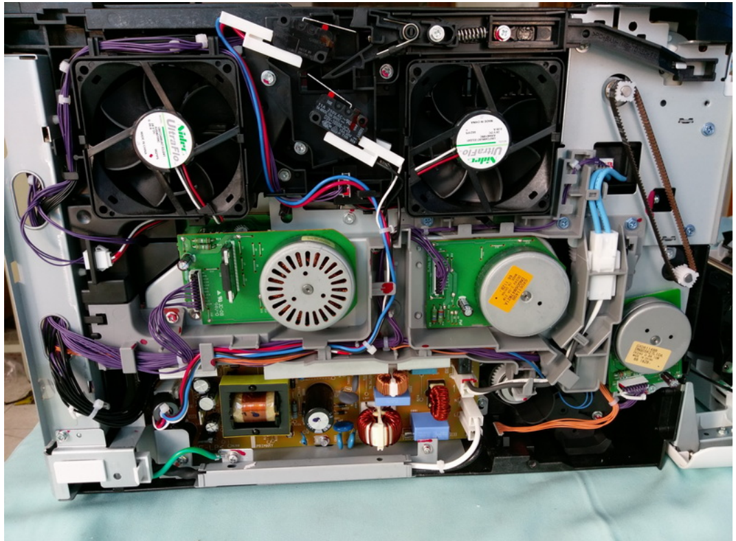
FIGURE 3 PRINTER (M/N: SP C262SFNW) COVER REMOVED #3
