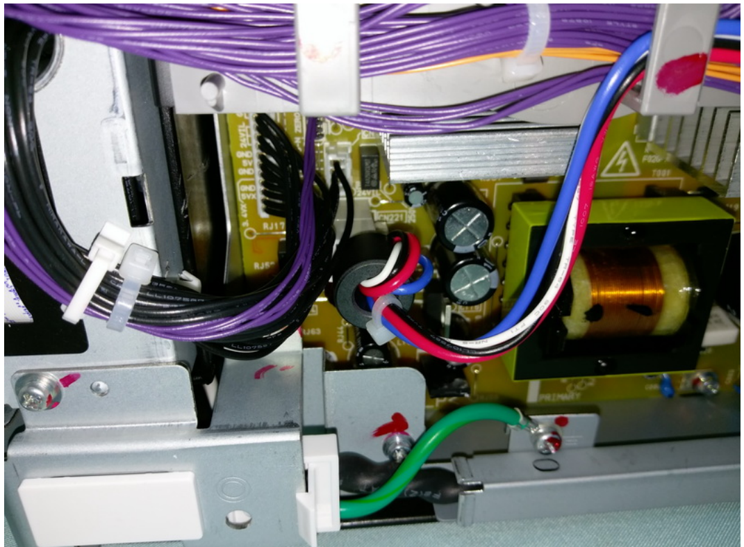
FIGURE 33 PRINTER (M/N: SP C262SFNW) DEBUG #2
