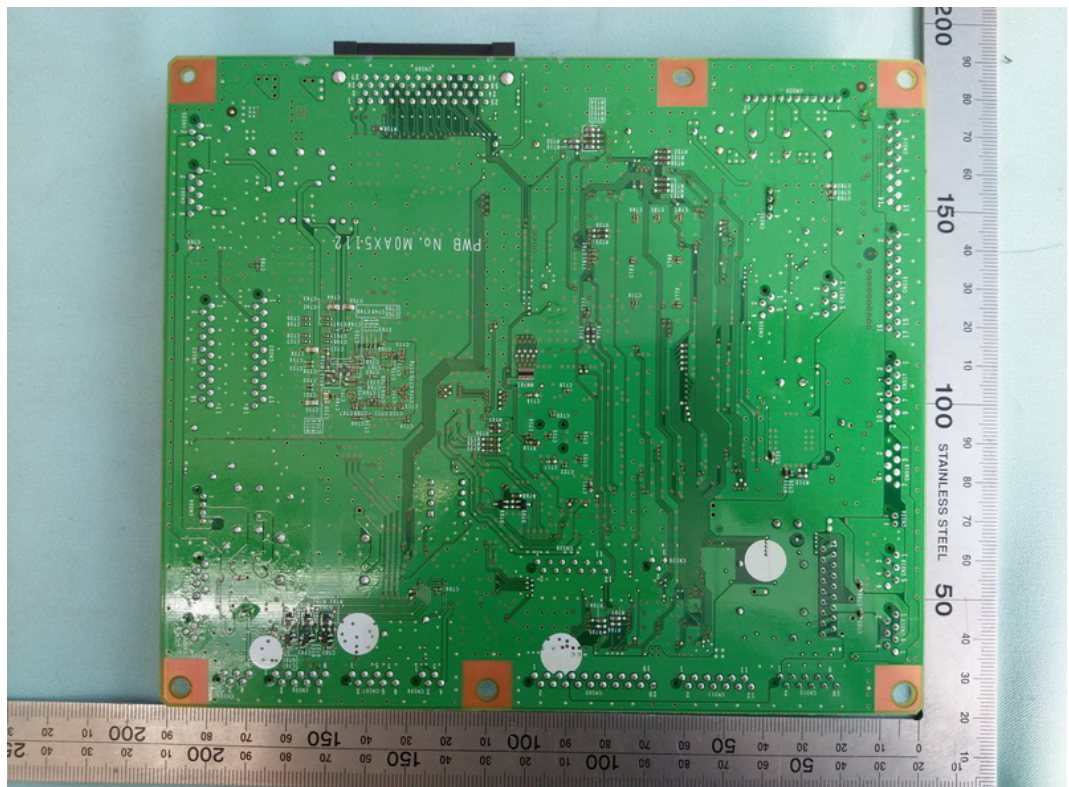
FIGURE 5 PRINTER (M/N: SP C262SFNW) MAIN BOARD (SOLDERED SIDE)
