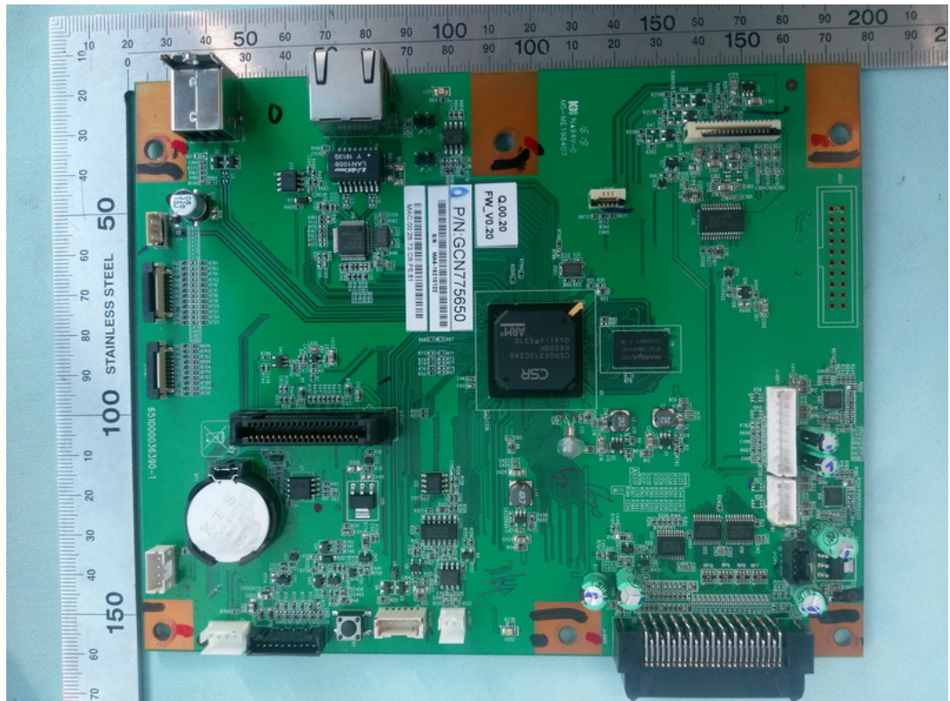
FIGURE 8 PRINTER (M/N: SP C262SFNW) SIGNAL BOARD (COMPONENT SIDE)
