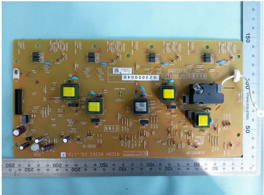
FIGURE 13 PRINTER (M/N: SP C262SFNW) POWER BOARD #2 (COMPONENT SIDE)
