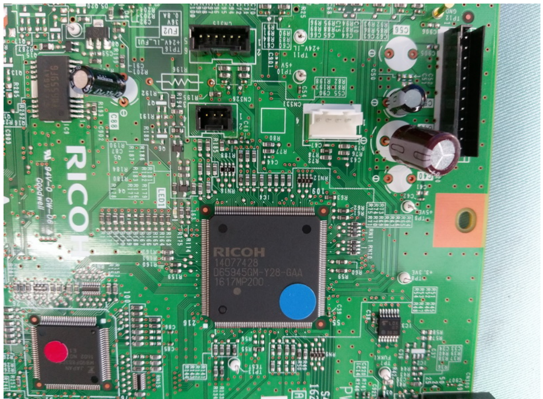
FIGURE 7 PRINTER (M/N: SP C262SFNW) CHIP #2 AND CRYSTAL #2 ON MAIN BOARD
