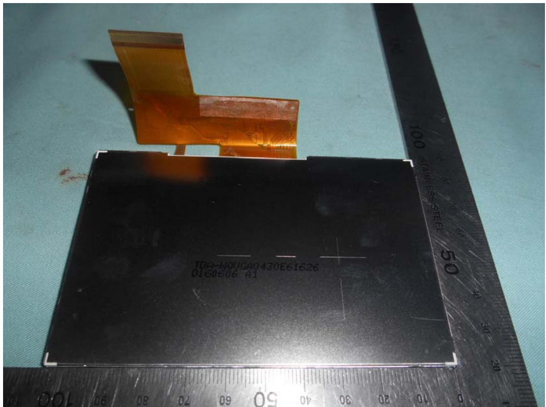
FIGURE 31 PRINTER (M/N: SP C262SFNW) PANEL BACK VIEW
