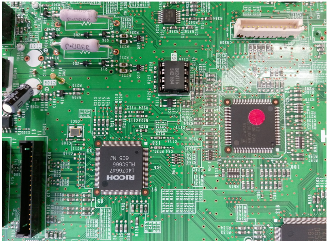
FIGURE 6 PRINTER (M/N: SP C262SFNW) CHIP#1 AND CRYSTAL#1 ON MAIN BOARD
