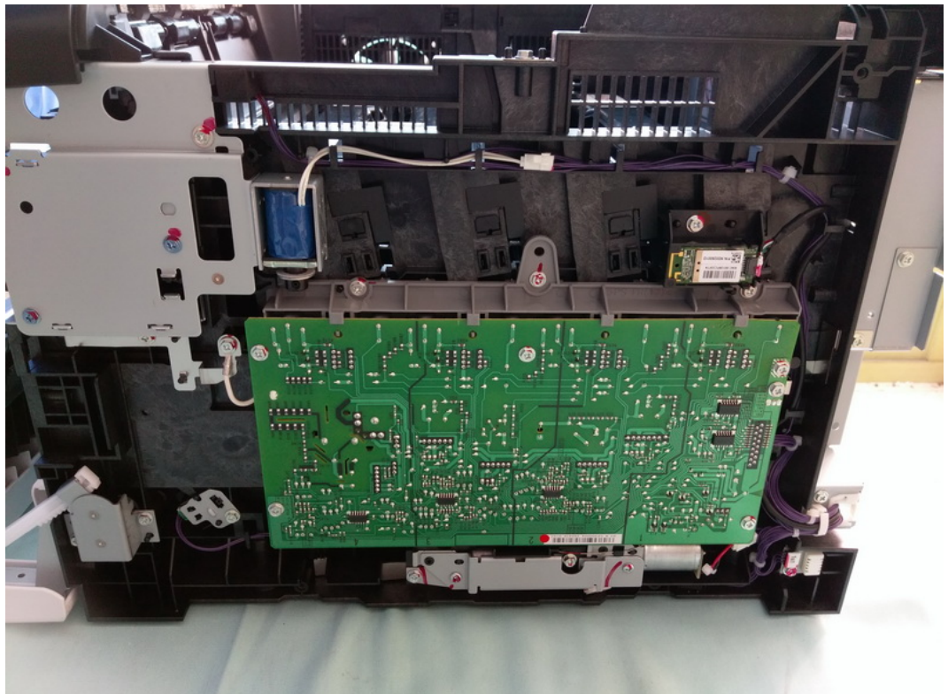
FIGURE 2 PRINTER (M/N: SP C262SFNW) COVER REMOVED #2
