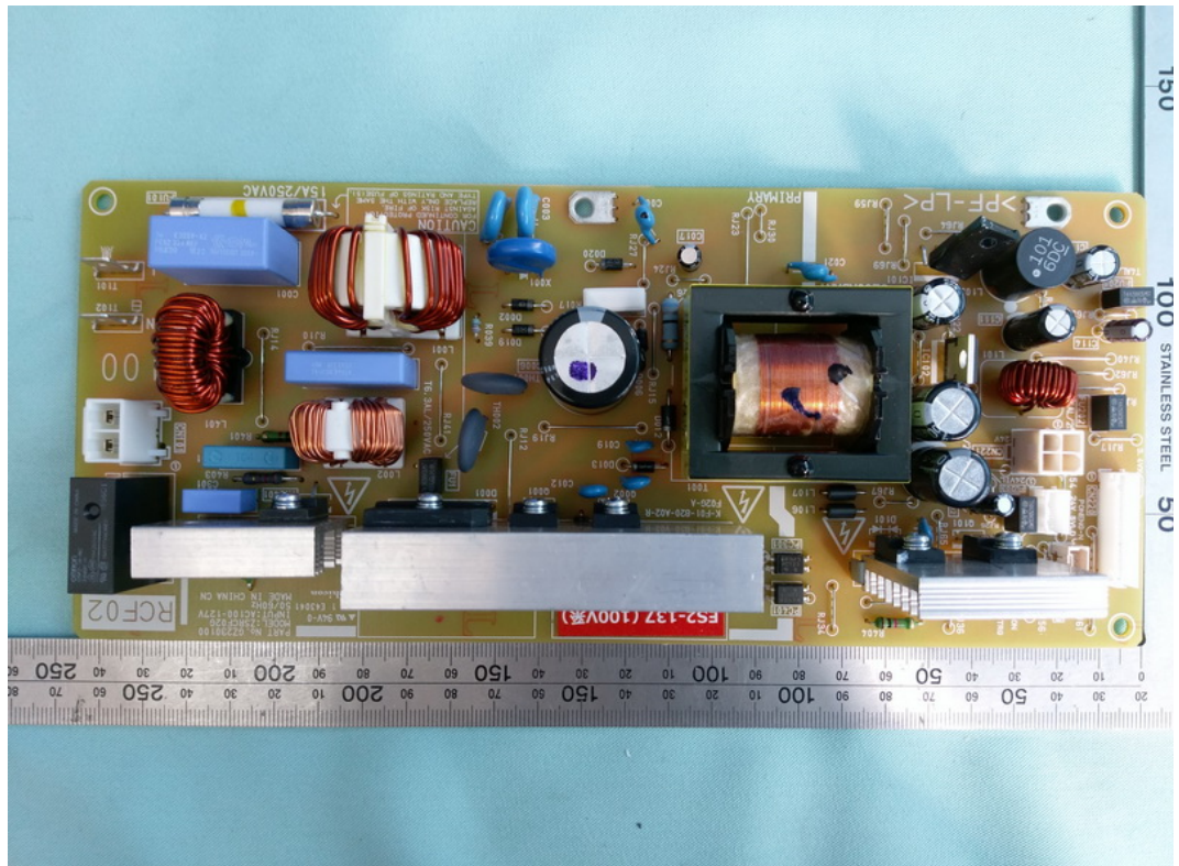
FIGURE 11 PRINTER (M/N: SP C262SFNW) POWER BOARD #1 (COMPONENT SIDE)
