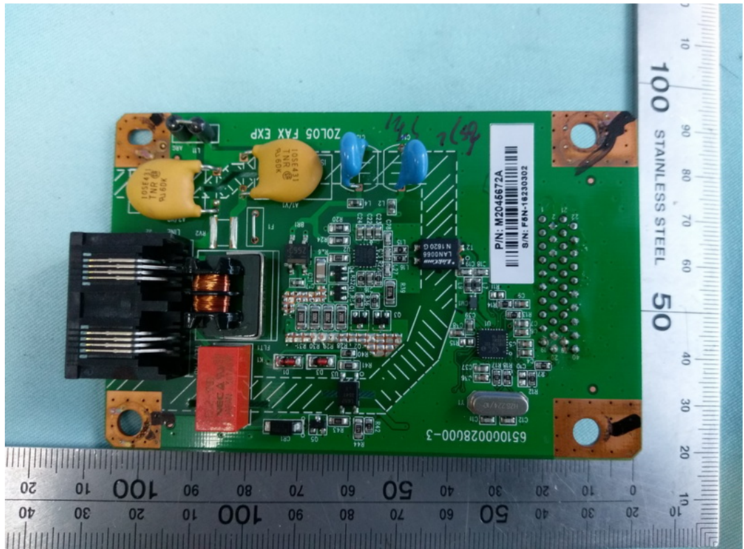
FIGURE 22 PRINTER (M/N: SP C262SFNW) POTS BOARD (COMPONENT SIDE)
