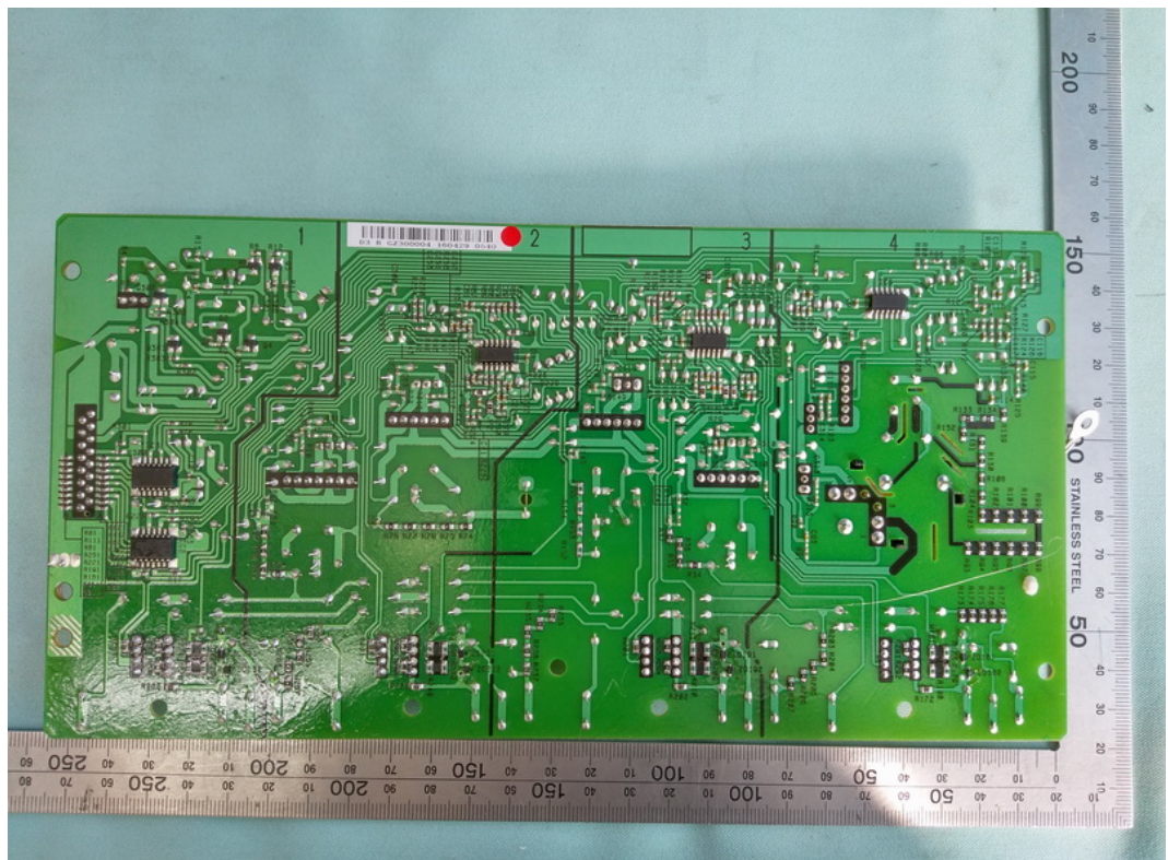
FIGURE 14 PRINTER (M/N: SP C262SFNW) POWER BOARD #2 (SOLDERED SIDE)
