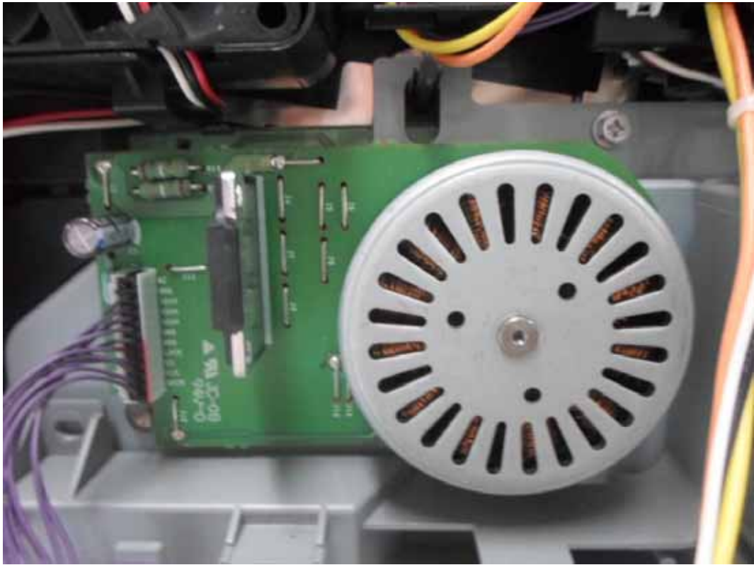
FIGURE 20 PRINTER (M/N: SP C252SF) MOTOR #3
