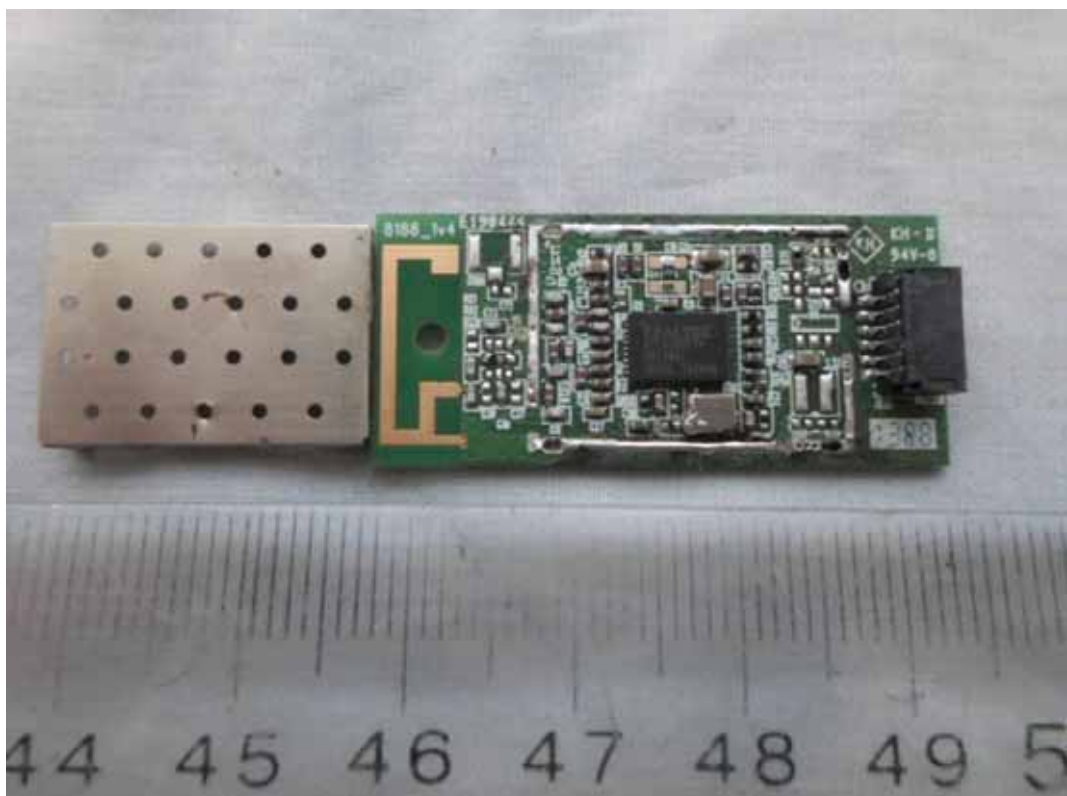
FIGURE 23 PRINTER (M/N: SP C252SF) WIFI BOARD (SHIELDED SHELL REMOVED)
