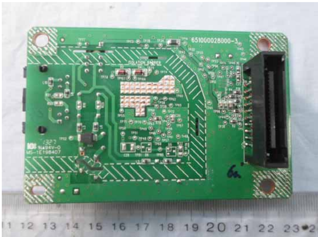
FIGURE 5 PRINTER (M/N: SP C252SF) POTS BOARD (SOLDERED SIDE)
