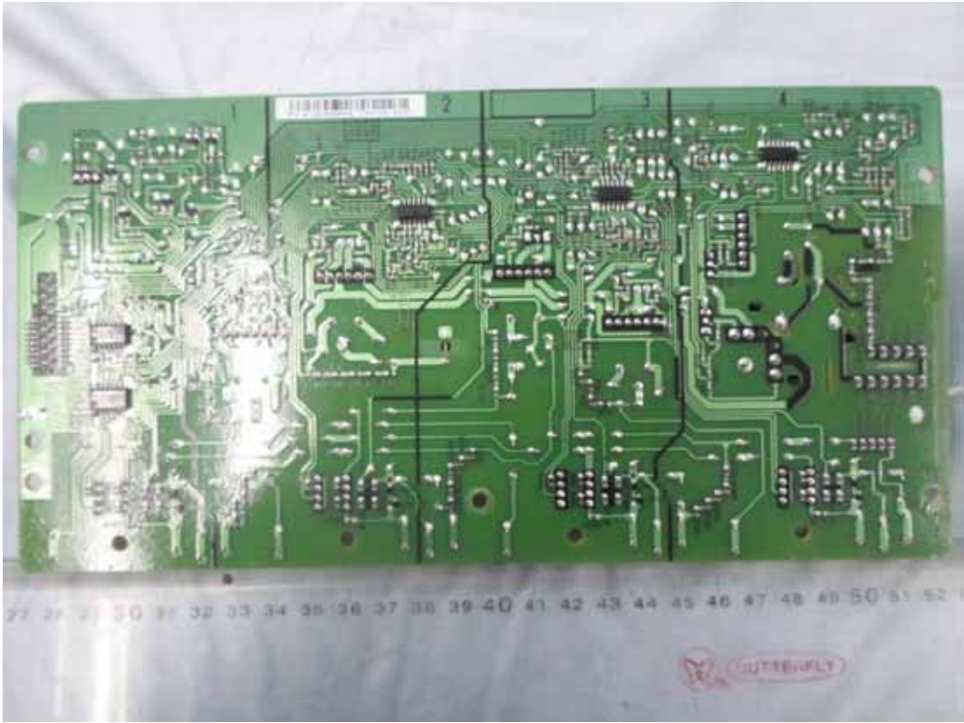
FIGURE 17 PRINTER (M/N: SP C252SF) POWER BOARD #2 (SOLDERED SIDE)
