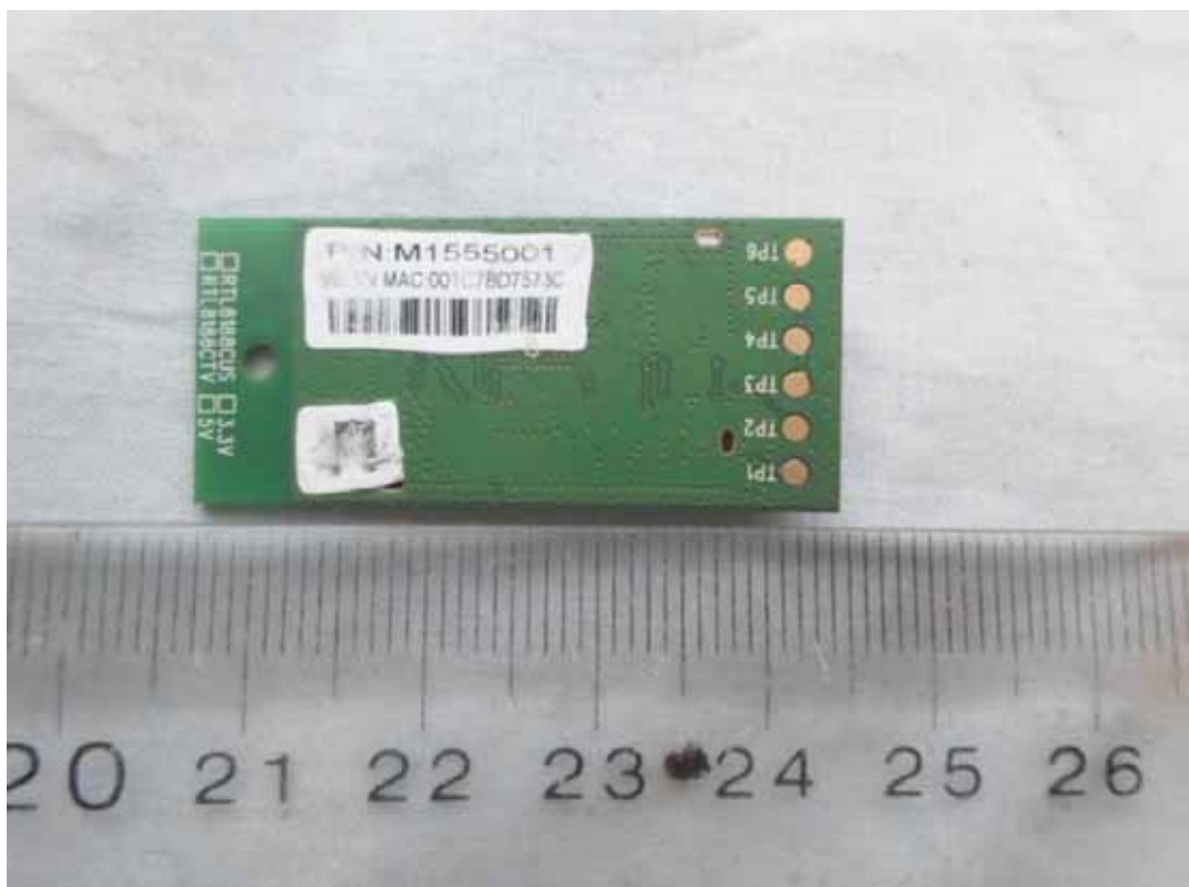
FIGURE 25 PRINTER (M/N: SP C252SF) WIFI BOARD (SOLDERED SIDE)
