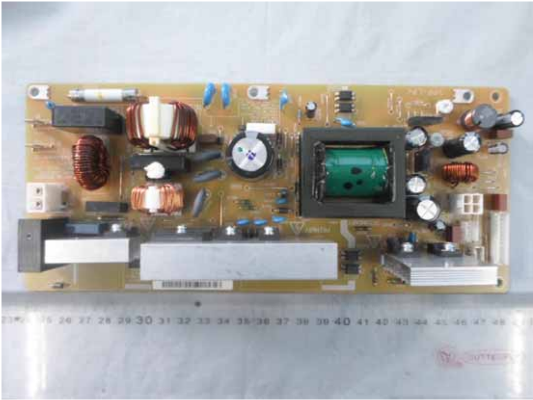
FIGURE 14 PRINTER (M/N: SP C252SF) POWER BOARD #1 (COMPONENT SIDE)
